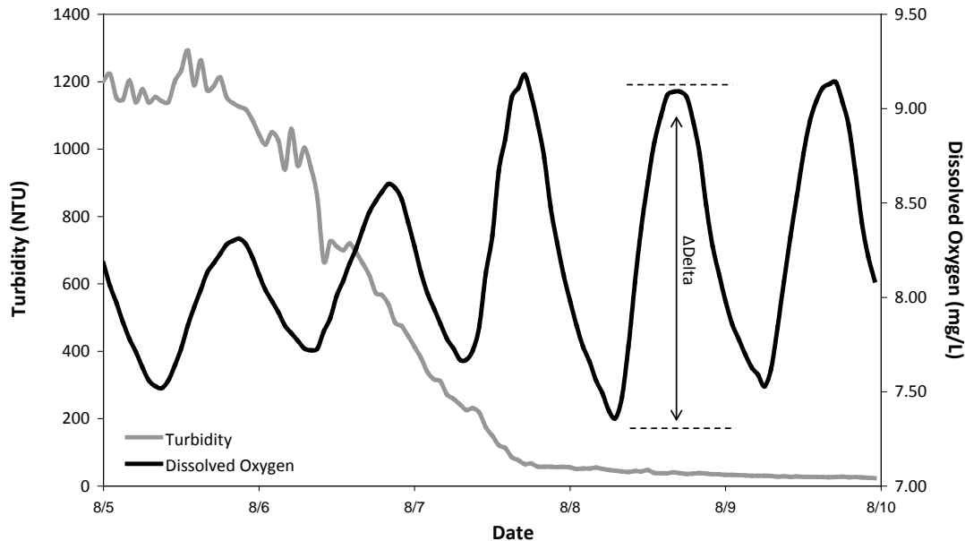
9 10 Figure 2-3. Influence of light attenuation on productivity in a Montana River.
