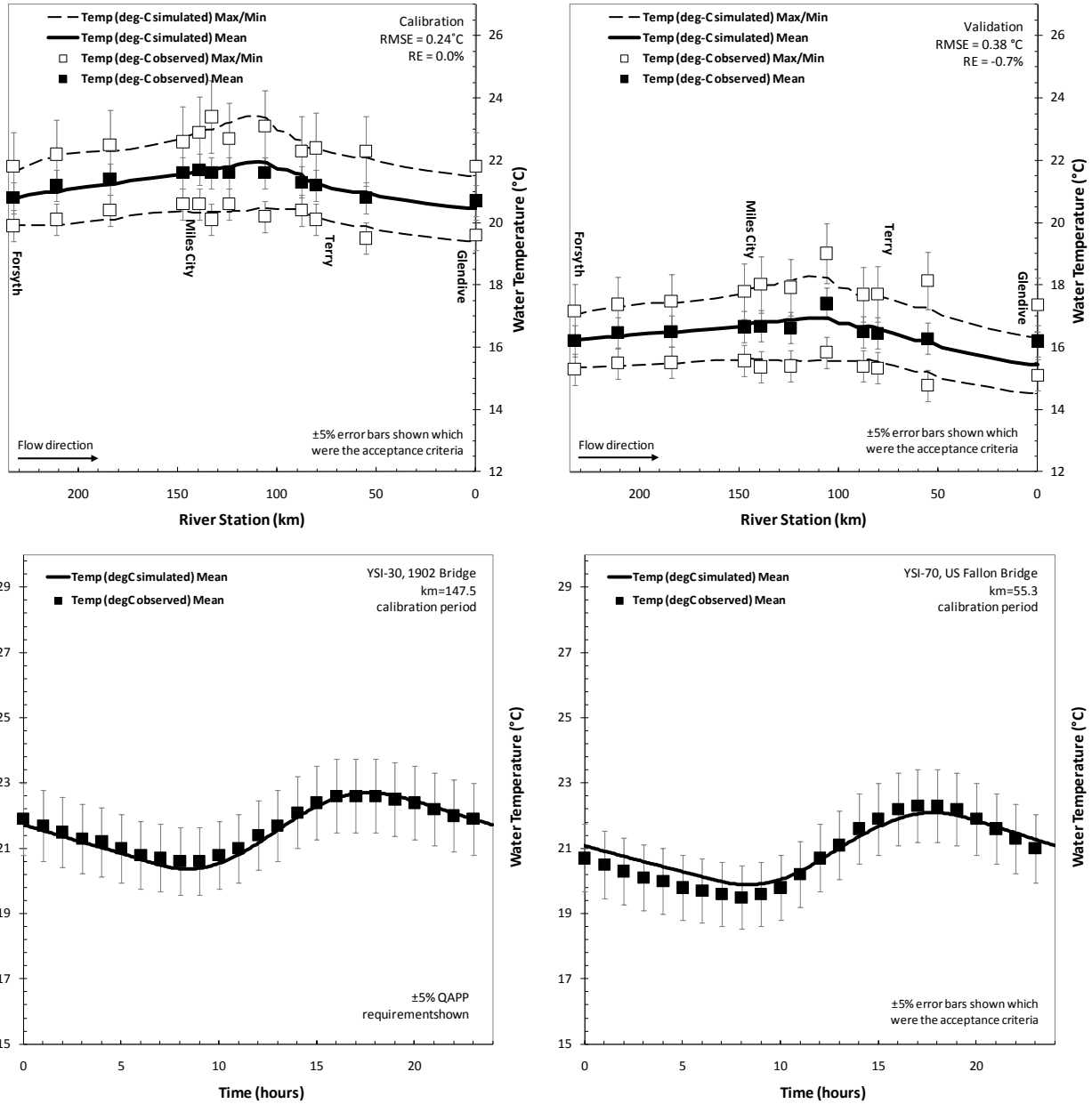
3 Figure 10-4. Water temperature simulation for the lower Yellowstone River during 2007.
