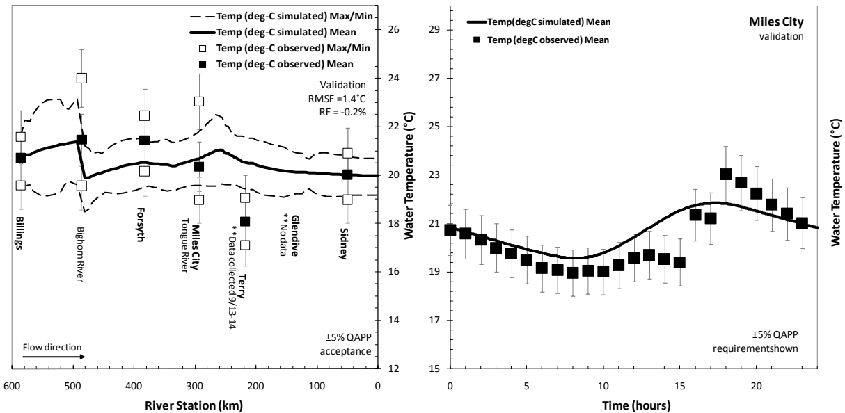
12 Figure 11-3. Temperature simulations for the Yellowstone River during 2000.
