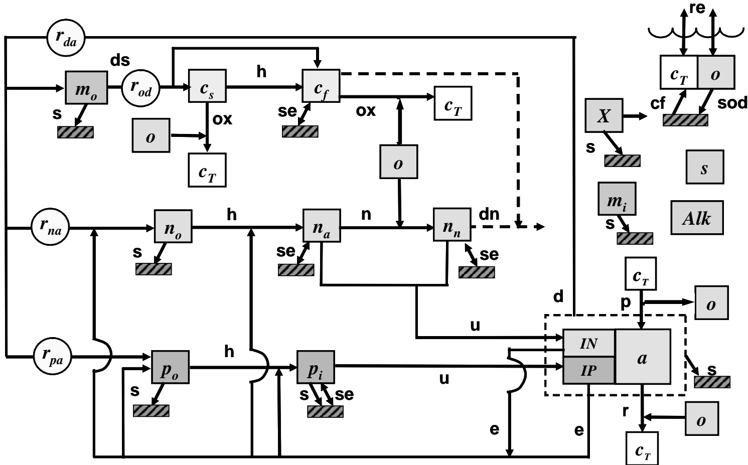
1 2 Figure 5-2. Diagram of model kinetics and mass transport processes in Q2K. 3 Redrawn from Chapra, 2008 (with permission). Kinetic processes are as follows: ds = dissolution, h = hydrolysis, ox = oxidation, n = nitrification, dn = 4 denitrification, p = photosynthesis, r = respiration, e = excretion, d = death, r = respiration. Mass transfer processes are: re = reaeration, s = settling, SOD = 5 sediment oxygen demand, se = sediment exchange, cf = inorganic carbon flux, u = uptake.
