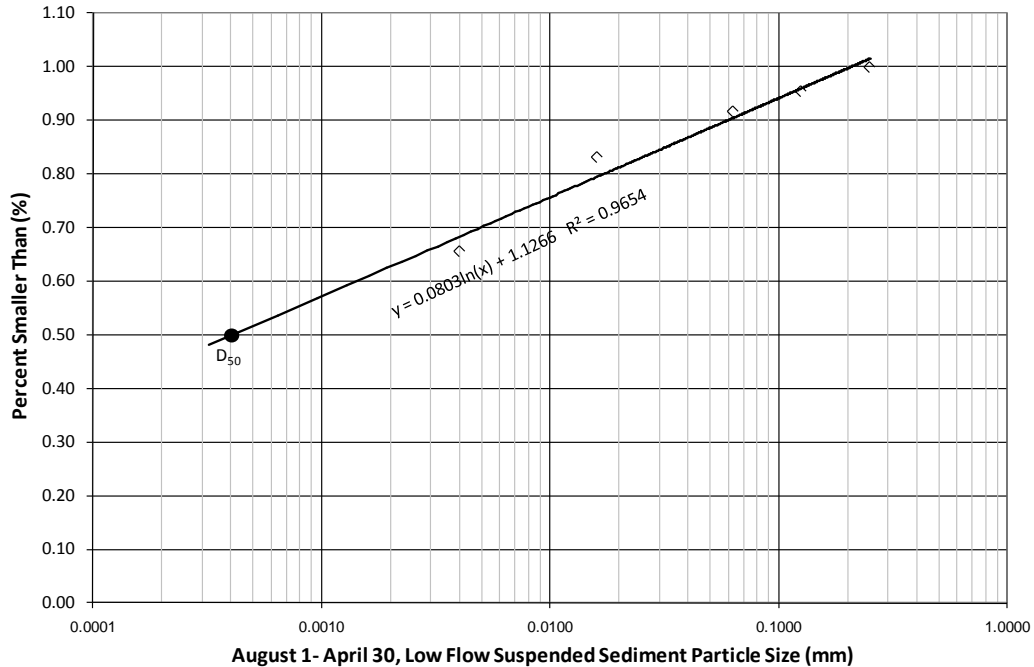
1 2 Figure 8-9. Suspended sediment particle size (mm) in Yellowstone River during low-flow conditions. 3 Data taken as average of fall diameter measurements at USGS 06295000 Yellowstone River at Forsyth MT and 4 USGS 06329500 Yellowstone River near Sidney MT.
