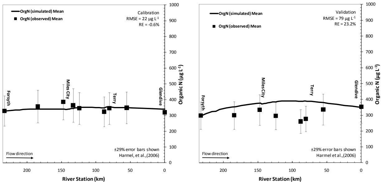
6 Figure 10-7. Total and organic N simulations for the Yellowstone River during 2007.
