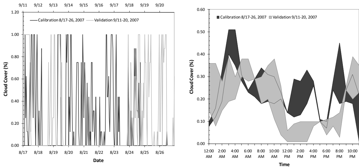
16 17 Figure 7-10. Hourly and repeating day cloud cover data for the lower Yellowstone River. 18 (Left panel) Cloud cover data for the 2007 period. (Right panel) Same but in a mean repeating day format. The 19 range of the climatic stations used in the modeling is shaded. 20
