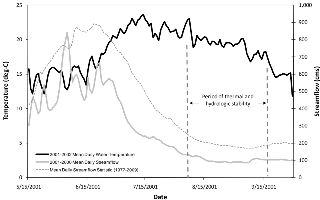
1 2 Figure 5-3. Typical occurrence of thermal and hydrologic stability in the Yellowstone River.
