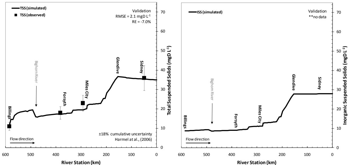
9 Figure 11-4. TSS simulations for the Yellowstone River during 2000.
