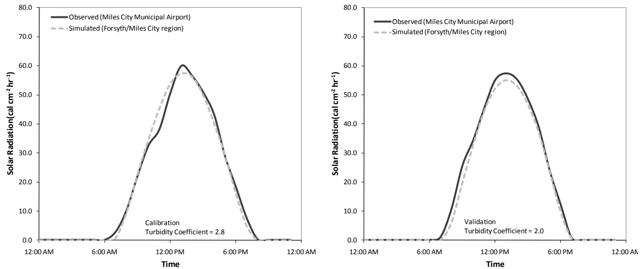
1 2 Figure 7-11. Simulated and observed solar radiation for the lower Yellowstone River. 3 (Left panel) Simulated and observed solar radiation for August 17-26, 2007 at Miles City Wiley Field. (Right panel) 4 Same but for September 11-20, 2007.
