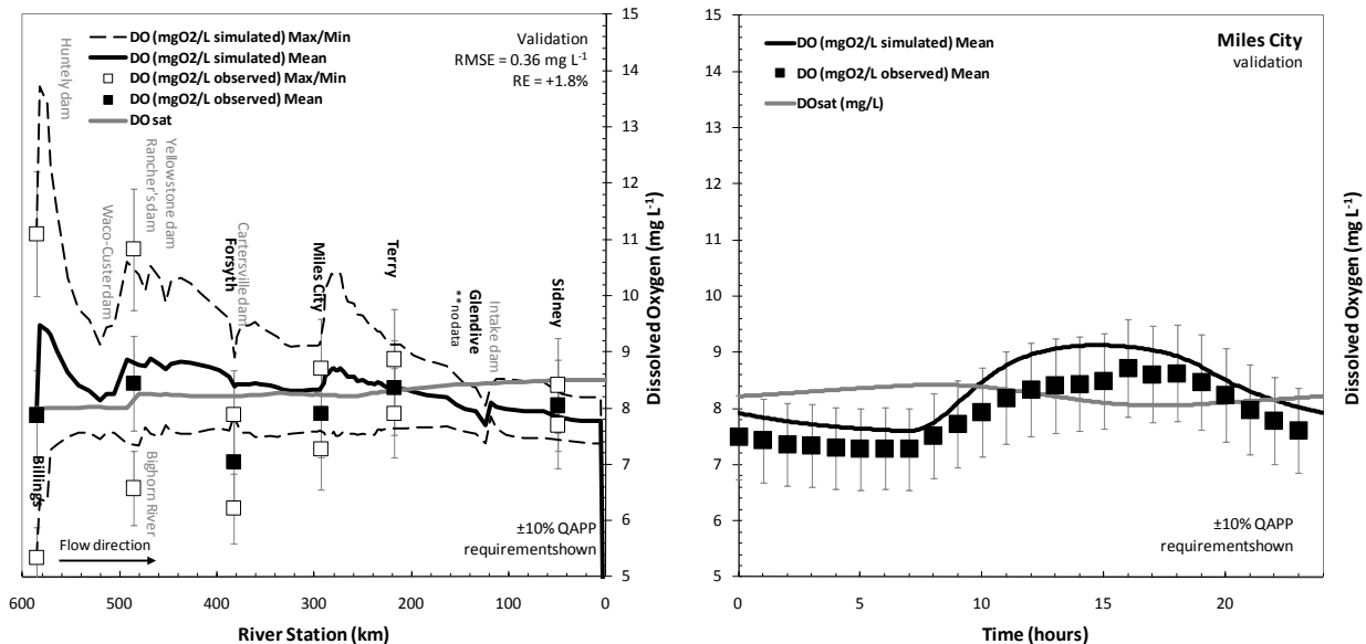
10 Figure 11-10. Dissolved oxygen simulations for the Yellowstone River during August 2000.
