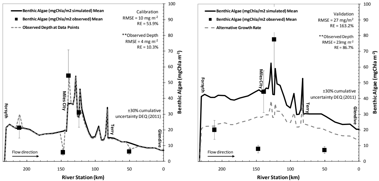
1 2 Figure 10-12. Simulated benthic algae Chla for the Yellowstone River during 2007.
