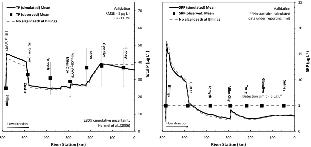
1 2 Figure 11-7. Phosphorus simulation for the Yellowstone River during August 2000. 3 (Left panel). Simulated and observed total phosphorus. (Right panel) Same but for SRP. Note that the USGS 4 observation site at Billings is directly upstream of the WWTP. Thus the large SRP actually occurs downstream of the 5 monitoring location.
