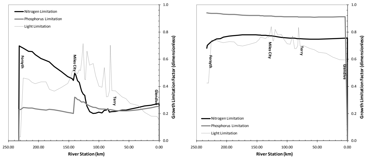
16 Figure 10-11. Nutrient and light limitation factors for the Yellowstone River during 2007.
