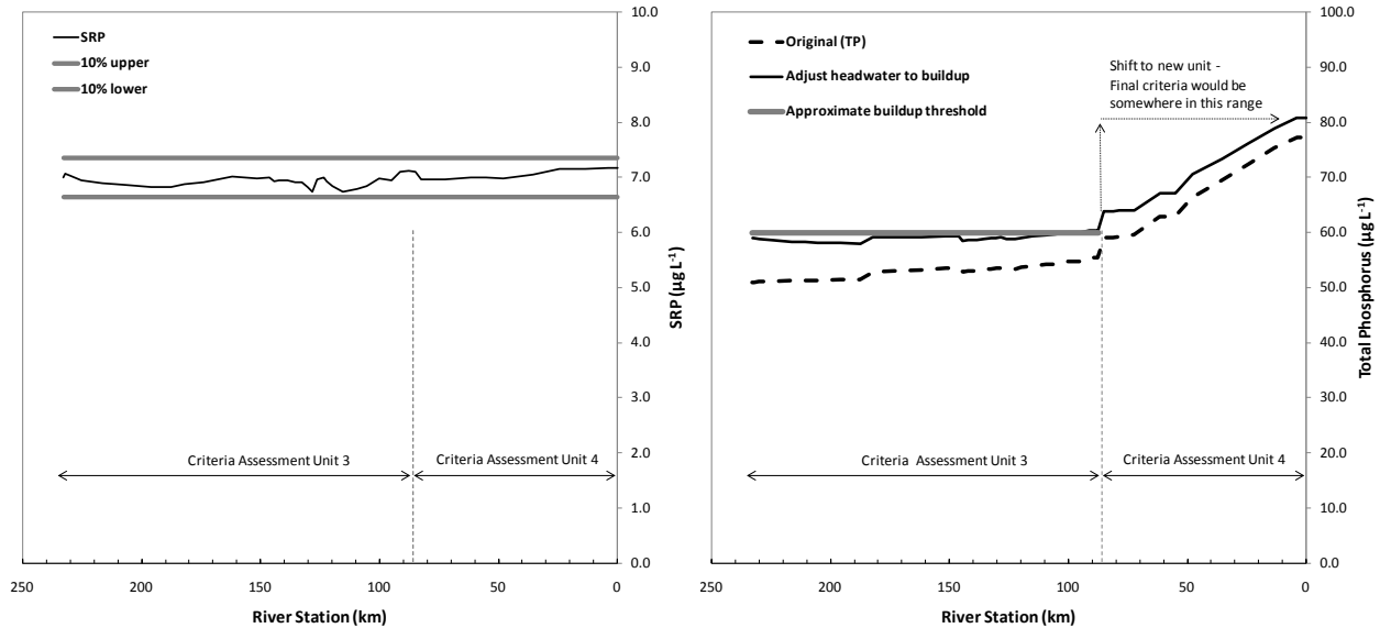
6 7 8 Figure 13-1. Example of the iterative procedure required to assign headwater boundary conditions. 9 (Left panel) Soluble phosphorus simulation shown for one of the ten TP optimizations (in this instance the target 10 SRP concentration was 7 µg L -1 ). (Right panel) Adjustment of headwater TP concentration (through adjustment of 11 OrgP) so that conditions reflect the approximate downstream buildup.
