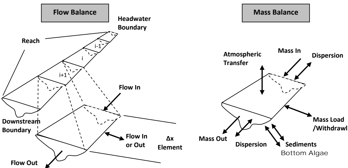
Figure 5-1. Conceptual representation of Q2K (redrawn from Brown and Barnwell, 2004).
