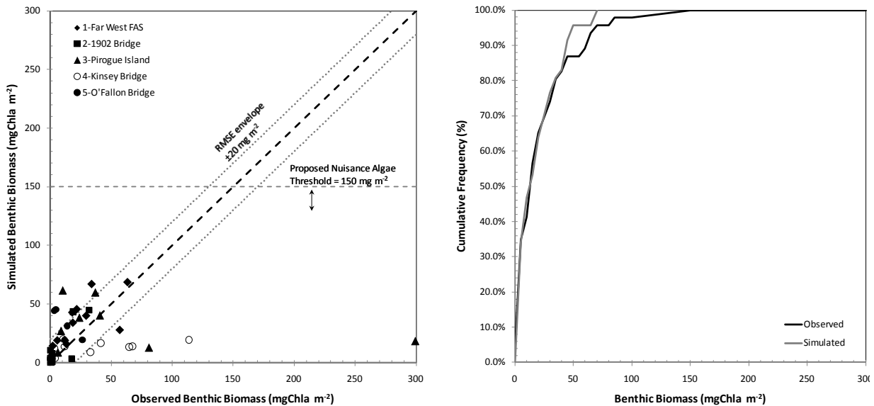
7 8 9 Figure 10-15. Benthic algal biomass lateral simulation reliability. 10 (Left panel) 1:1 plots of model simulations for the calibration period. A RMSE envelope is shown which represents 11 a plausible margin of safety to account for simulation error as discussed previously. (Right panel) Cumulative 12 frequency plot of simulated and observed benthic algal biomasses for the August 2007 period indicating relatively 13 consistent simulation of lower biomasses and tendency to underestimate higher biomasses. 14
