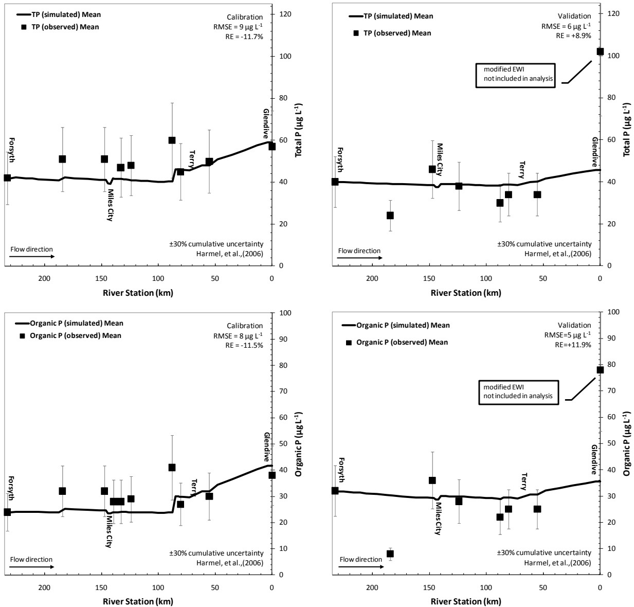
8 9 Figure 10-9. Total and organic phosphorus simulations for the Yellowstone River during 2007.
