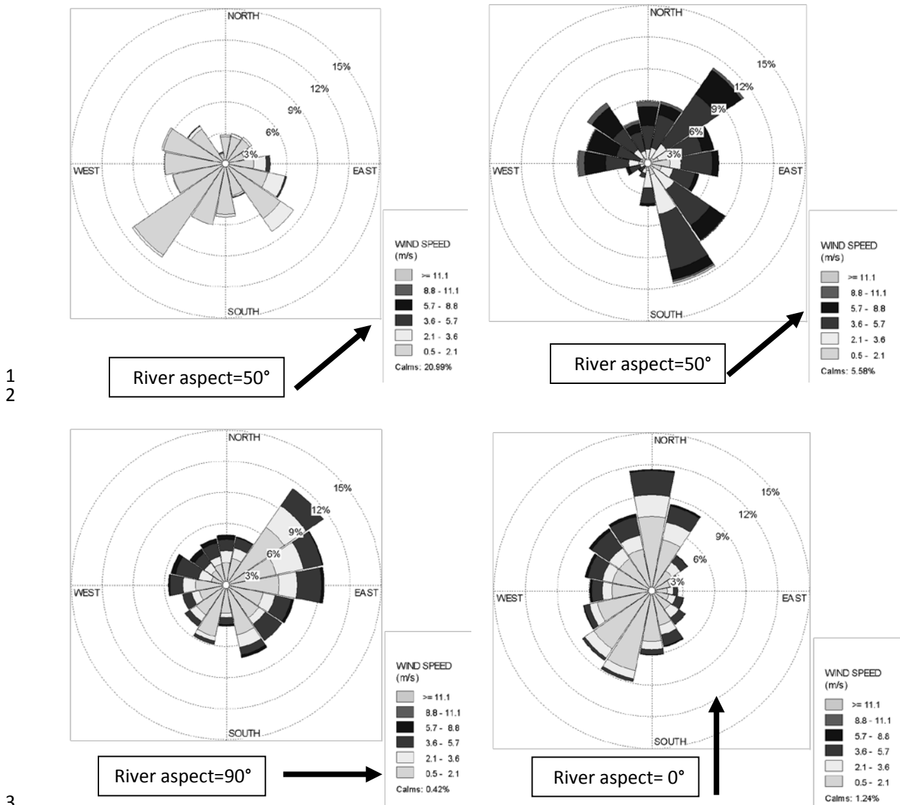
3 4 5 Figure 12-8. Wind Rose data on the lower Yellowstone River.
