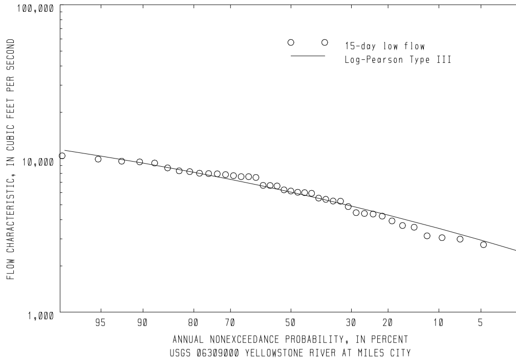
1 2 3 Figure 12-5. Log-Pearson Type III low-flow frequency curve for the Yellowstone River at Miles City. 4
