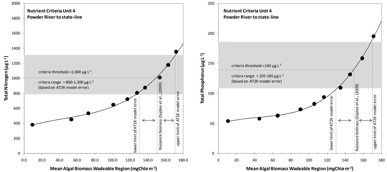
Figure 13-5. Non-linear response relationship between nutrients and benthic algae. (Left panel) Most limiting benthic algae wadeable response to TN in Criteria Assessment Unit 4. (Right panel) Same but for TP. Recreational use biomass thresholds are based on Suplee, et al., (2009) and reflect the mean density in the wadeable zone (see further discussion in Section 13.3.2 ). Existing criteria are shown as the independent variable (x) and corresponding nutrient concentrations as dependent variable (y). Note: The grey shaded area reflects the uncertainty in the model prediction based on model errors determined in Section 10.0 . TN and TP criteria in Unit 4 are recommended at \approx 1,000 \mu\text{g TN L}^{-1} and 140 \mu\text{g TP L}^{-1} in this region.
