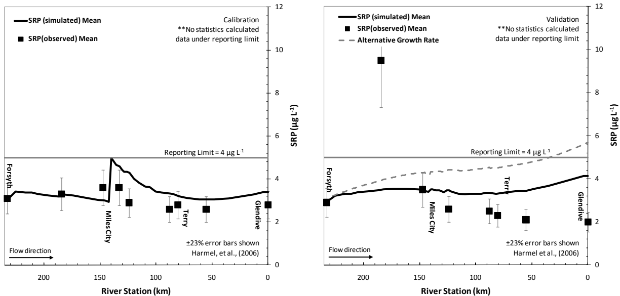
12 Figure 10-10. Soluble phosphorus simulations for the Yellowstone River during 2007.
