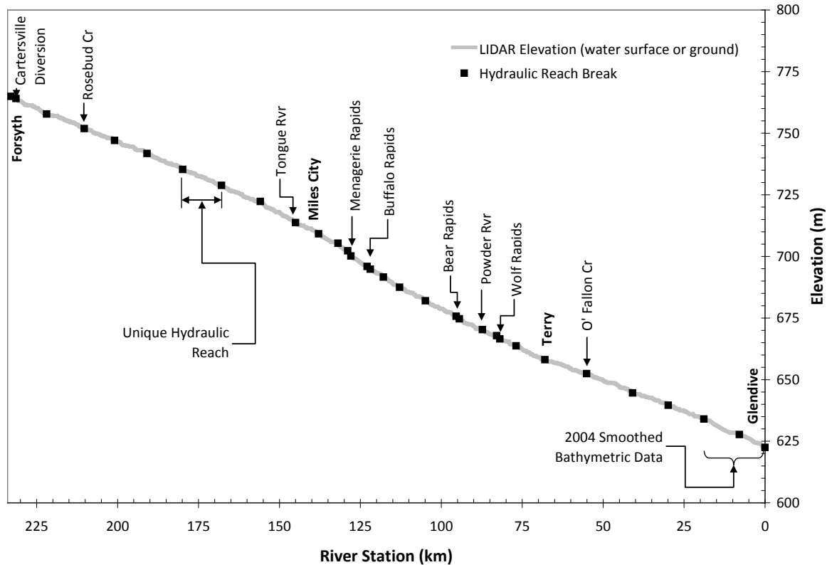
1 2 Figure 7-1. Longitudinal profile of the Yellowstone River.
