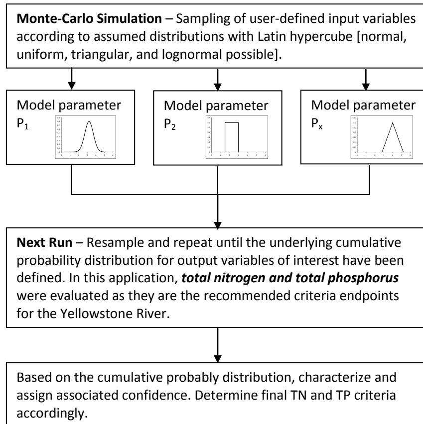
38 Figure 14-1. Example of Monte Carlo simulation procedure for Yellowstone River.
