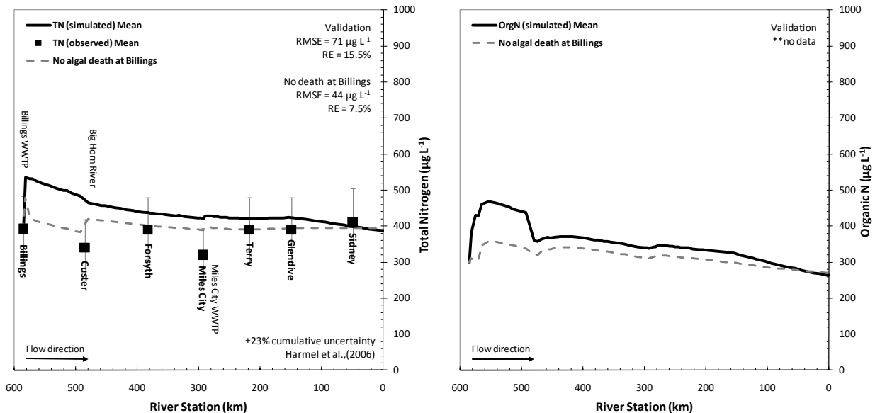
8 9 Figure 11-5. Total and organic N simulations for the Yellowstone River during August 2000.
