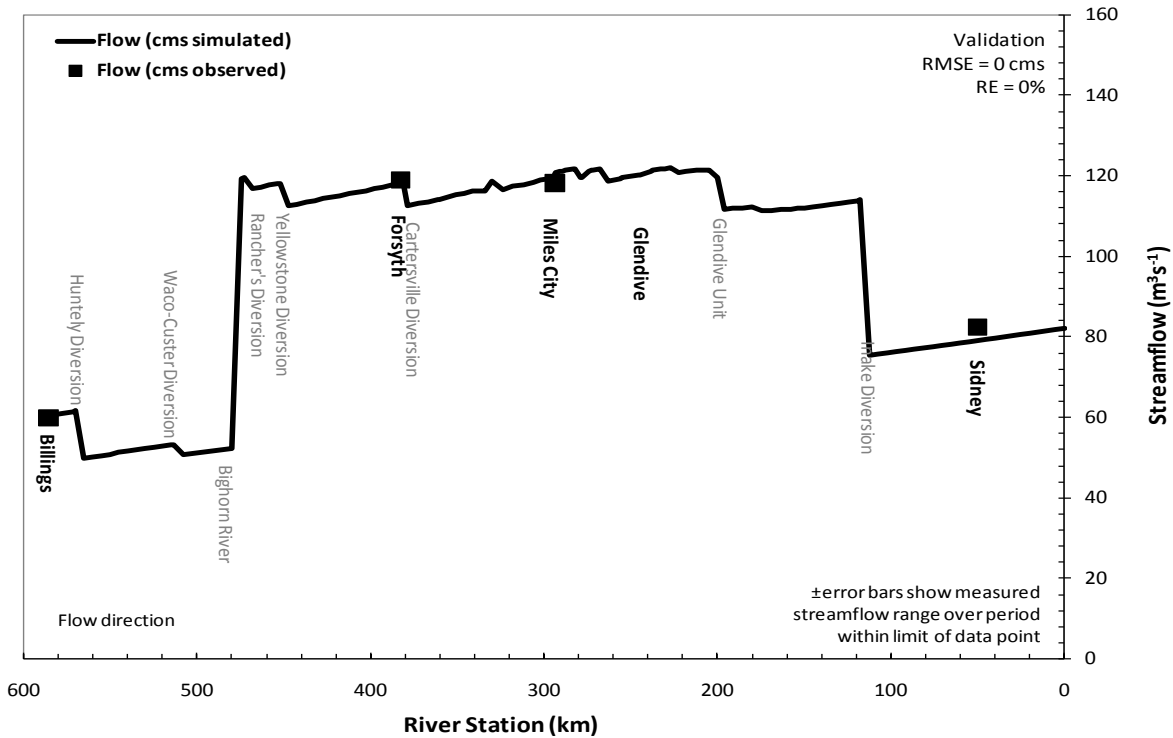
1 2 Figure 11-1. Simulated and observed streamflow for the Yellowstone River during 2000. 3
