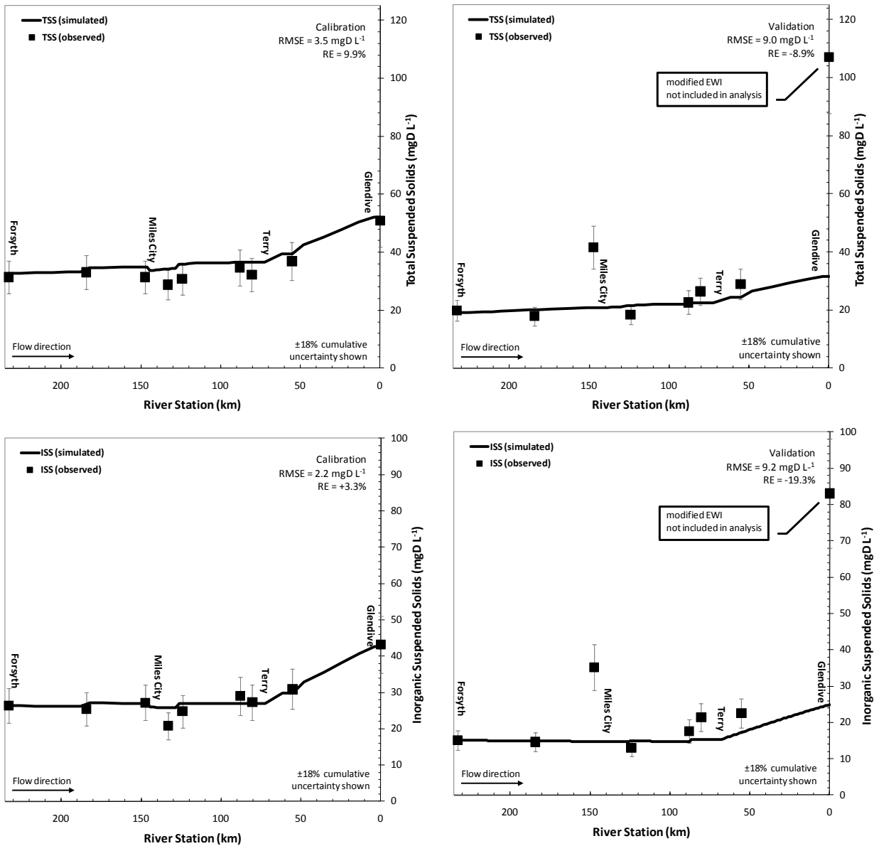
5 6 7 Figure 10-5. TSS and ISS simulations for the lower Yellowstone River during 2007. 8 (Top left/right panel) Simulated and observed TSS values for the August and September calibration and validation 9 period. (Bottom left/right panel) Same but for ISS. The ±18% cumulative uncertainty is based on Harmel, et al., 10 (2006).
