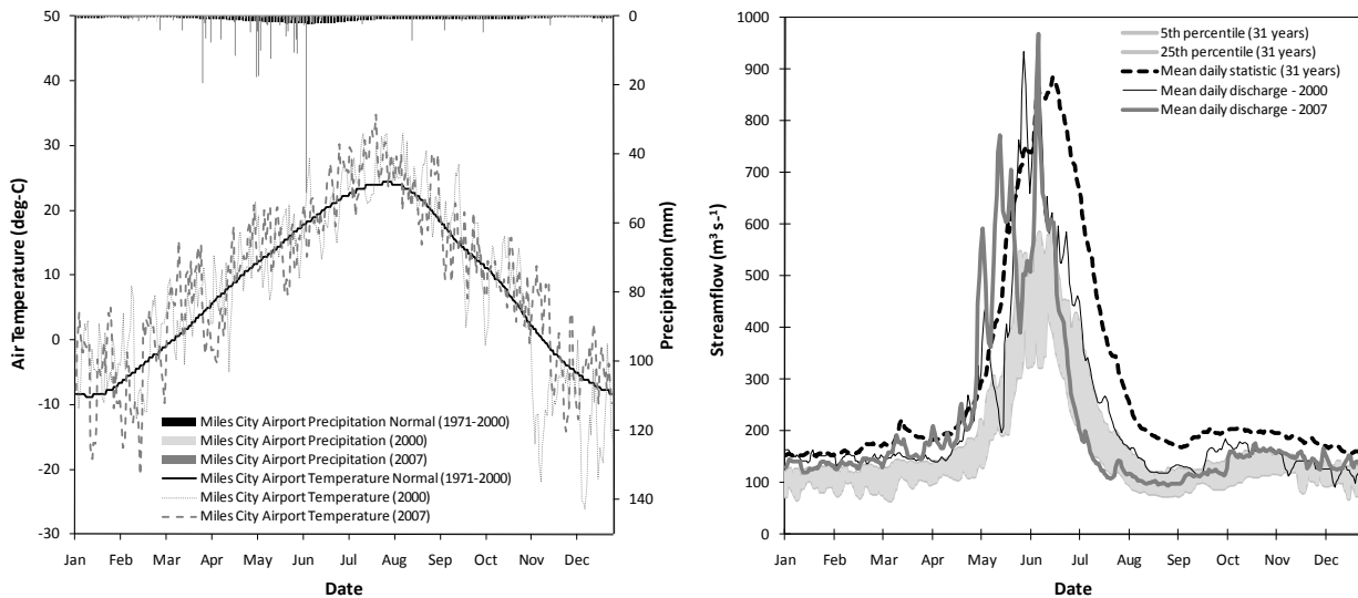
11 Figure 6-3. Conditions encountered during the 2000 and 2007 field data collection efforts. 12 (Left panel) Climatological data. (Right panel) Streamflow hydrology.
