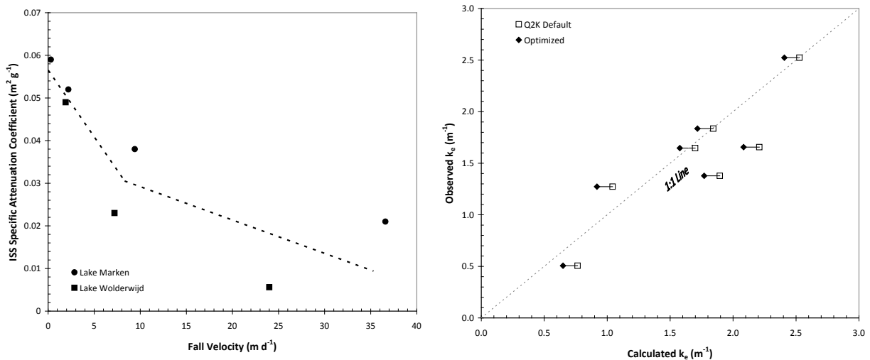
12 13 Figure 8-10. Optimized partial extinction coefficients for the remaining coefficients ( \alpha_i, \alpha_o, \alpha_p & \alpha_{pn} ). 14 (Left) Relationship between fall velocity and inorganic suspended solids partial attenuation coefficient ( \text{m}^2 \text{ g}^{-1} ) 15 based on data from (Blom, et al., 1994). (Right) Optimization of remaining partial attenuation values for detritus 16 and phytoplankton showing the relative shift toward the 1:1 line.
