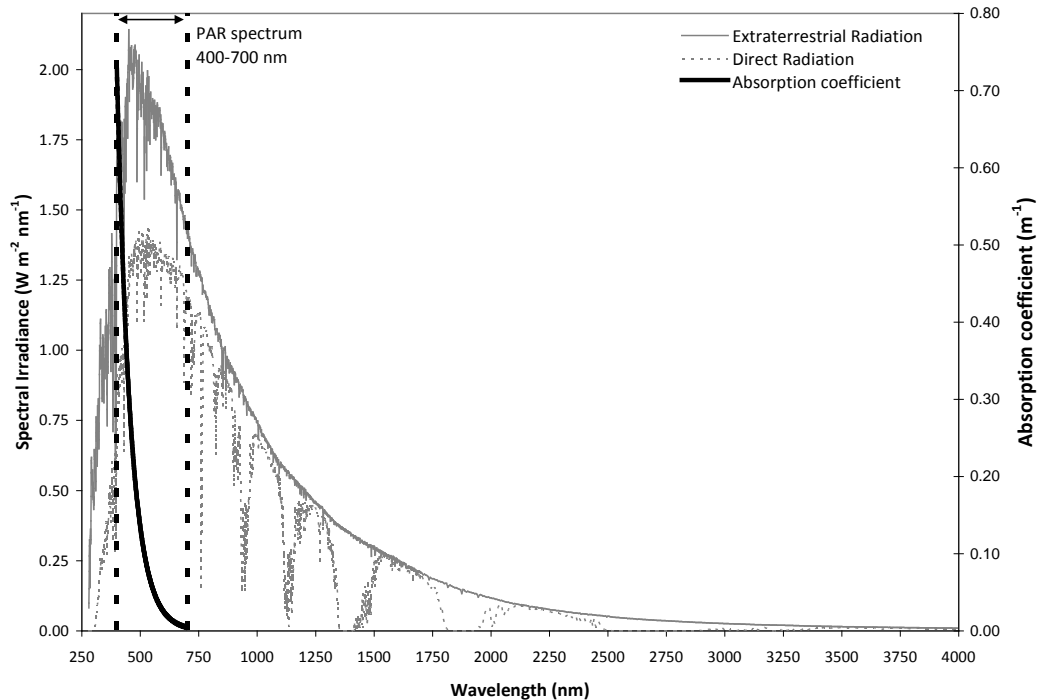
1 2 Figure 8-8. ASTM reference spectra used to evaluate the net absorption coefficient for color.
