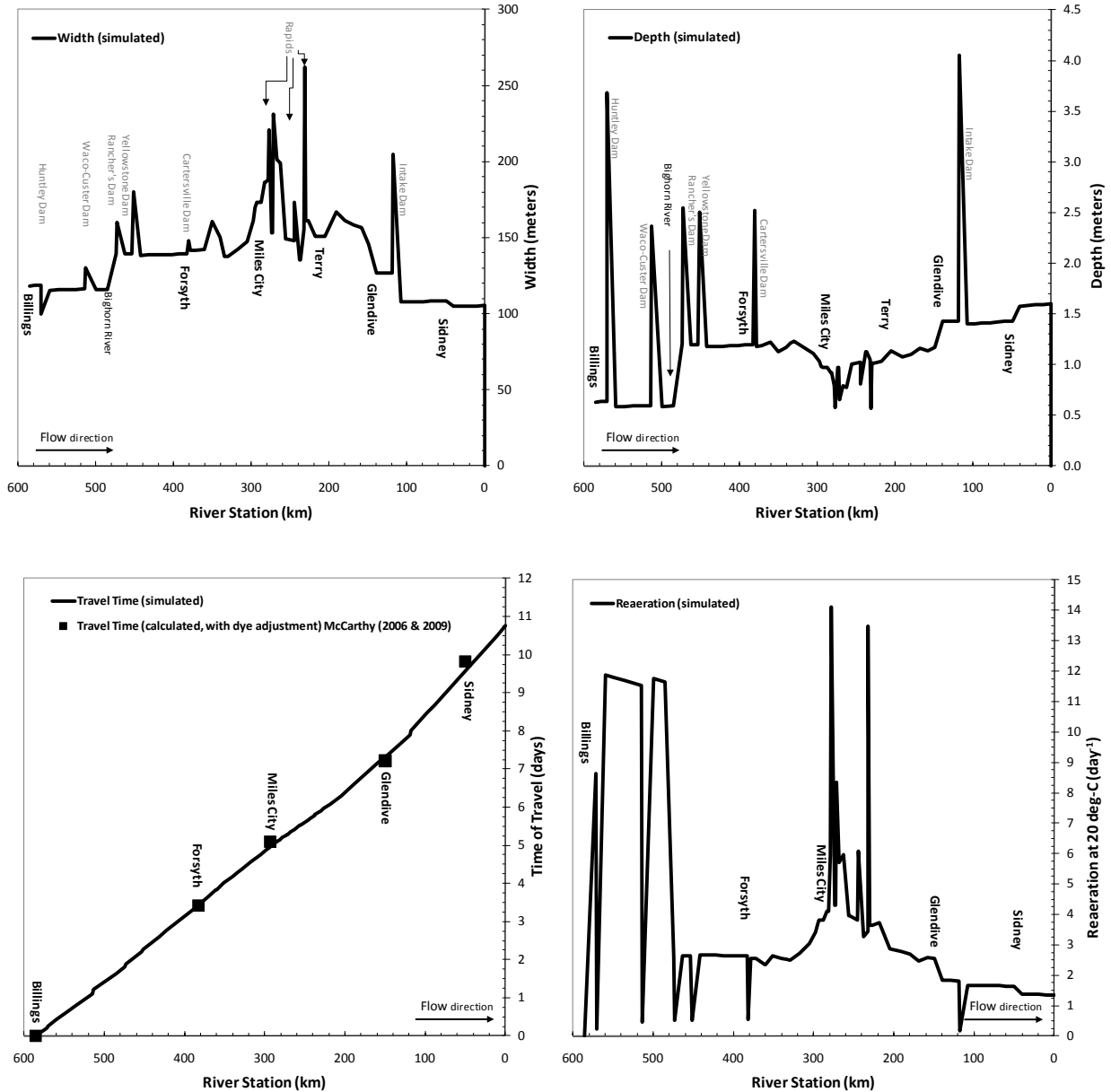
Figure 11-2. Mass transport indicators for the lower Yellowstone River during 2000. (Top left/right panel). Simulated width and depth. (Bottom left/right panel) Travel-time and reaeration.
