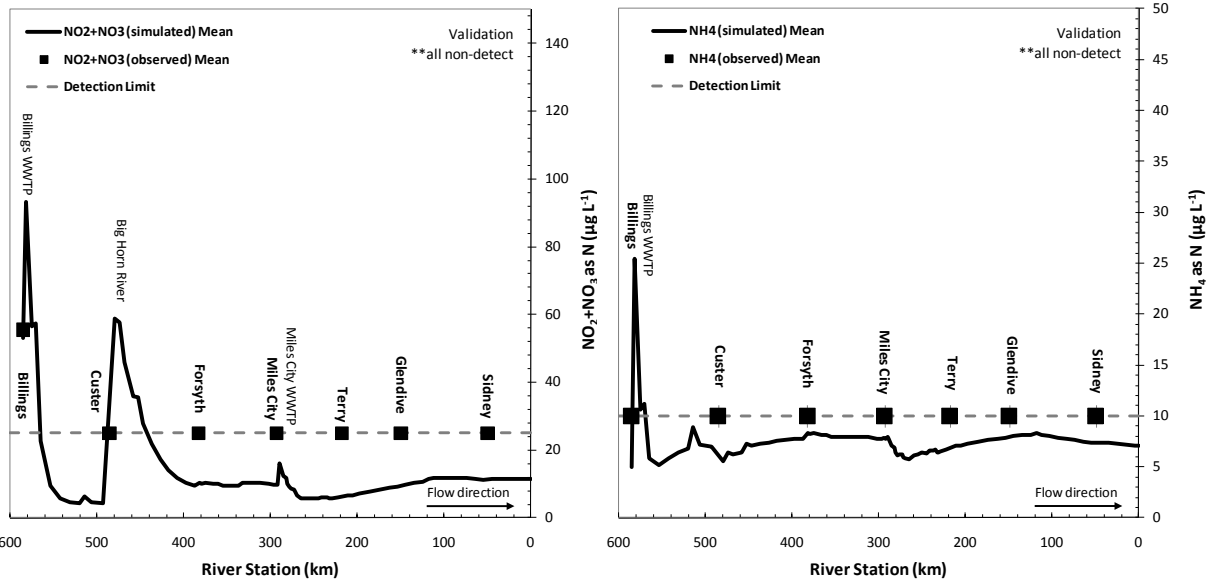
1 2 Figure 11-6. Nitrogen simulations for the Yellowstone River during August 2000. 3 (Left panel). Simulated and observed nitrate. (Right panel) Same but for ammonia. Both of the soluble N plot data 4 are below the detection limits referenced by the dotted line.
