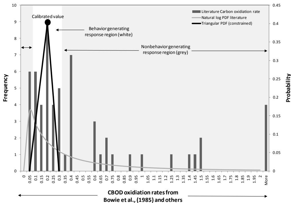
19 20 21 Figure 14-3. Example PDF assignment for model rate coefficients on the Yellowstone River.
