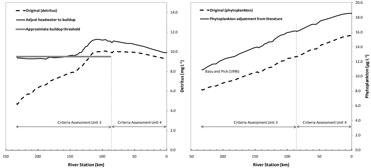
1 2 3 Figure 13-2. Consideration of headwater detritus and phytoplankton concentrations.
