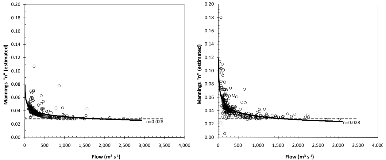
1 2 Figure 7-5. Estimated variation of Manning's n with flow for the Yellowstone River.
