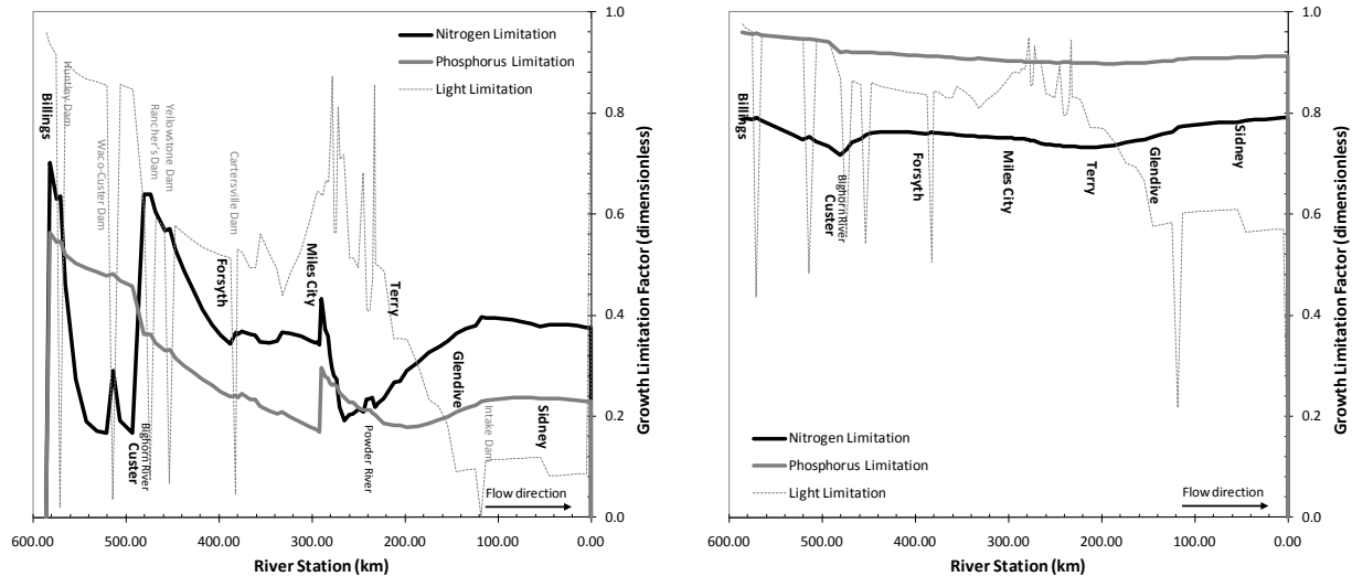
1 2 Figure 11-8. Nutrient and light limitation factors for the Yellowstone River during 2000.
