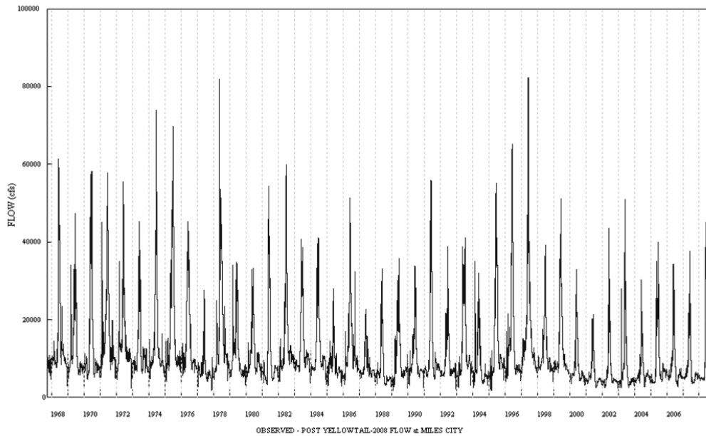
4 Figure 12-3. Period of record used in development of low-flow frequency curves for Miles City.
