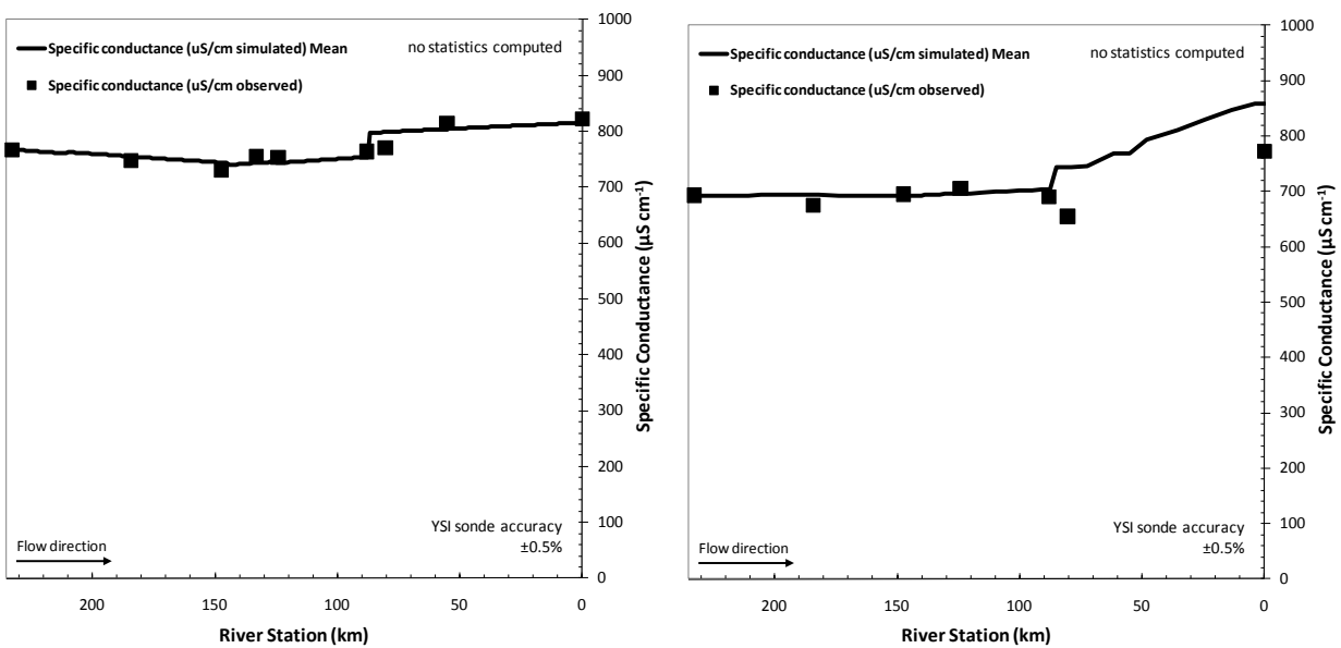
14 Figure 10-21. Conductivity simulations for the Yellowstone River during 2007.
