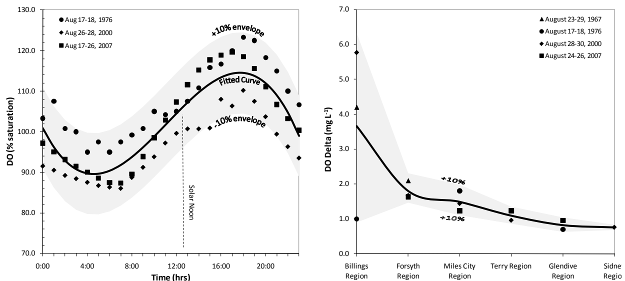
14 15 Figure 6- 2. Dissolved oxygen data on the Yellowstone River for August 1967, 1976, 2000, and 2007. 16 (Left panel) Typical diurnal pattern at Forsyth, MT over the August 1976, 2000, and 2007 period. A fitted curve is 17 shown along with as \pm 10\% saturation envelope. (Right panel) Longitudinal diurnal fluctuation in DO (i.e. max-min) 18 over all years. Envelope shown as \pm 10\% of the reported maximum or minima.
