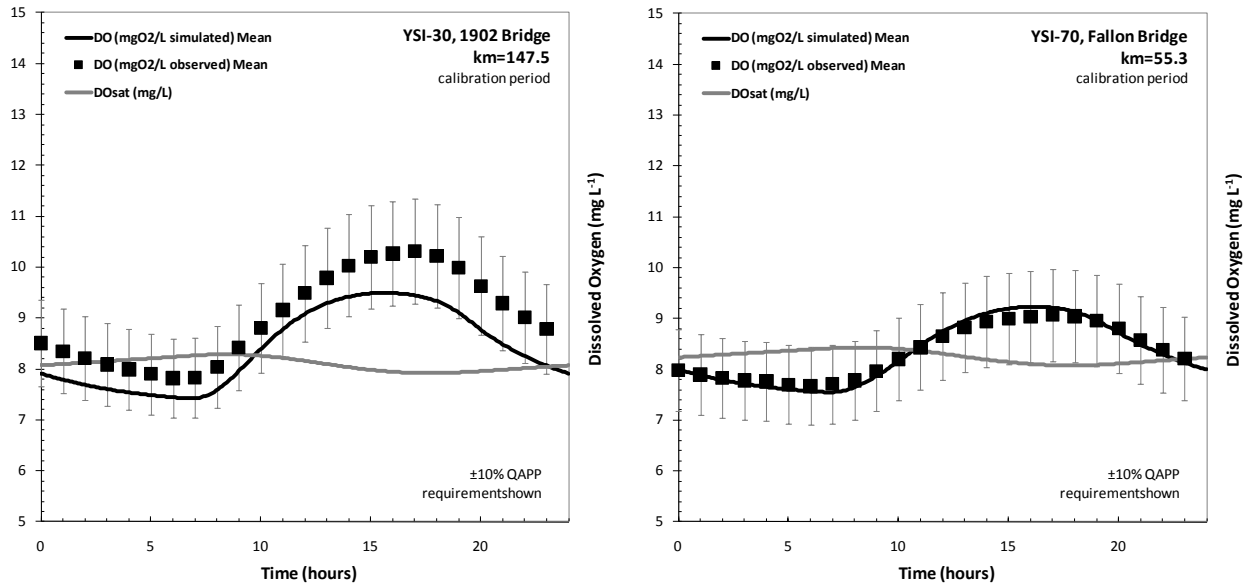
1 2 Figure 10-17. DO simulations for the lower Yellowstone River during 2007.
