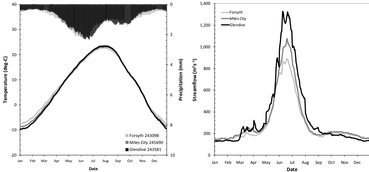
4 Figure 4-4. Mean daily normals for the lower Yellowstone River.
