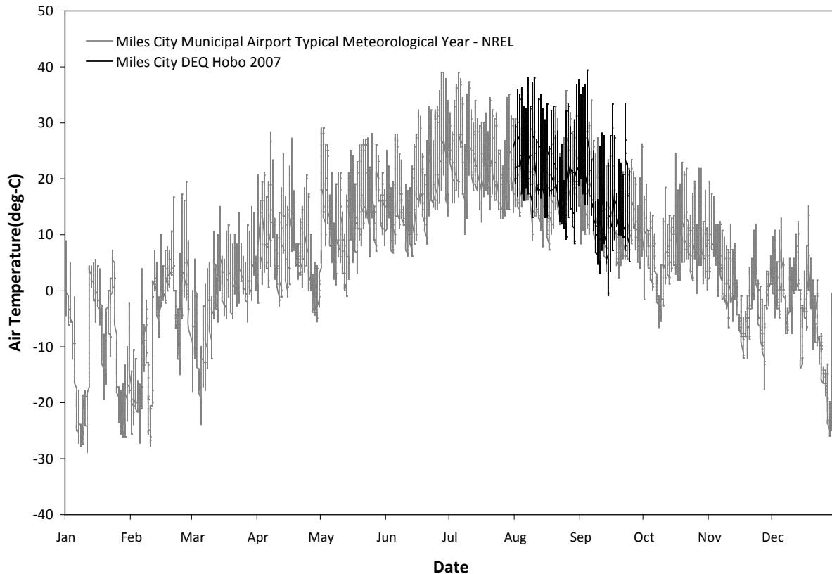
12 13 Figure 12-6. Example TMY air temperature plot for 742300 Miles City Municipal Airport. 14 Field observations from 2007 are shown for reference purposes.
