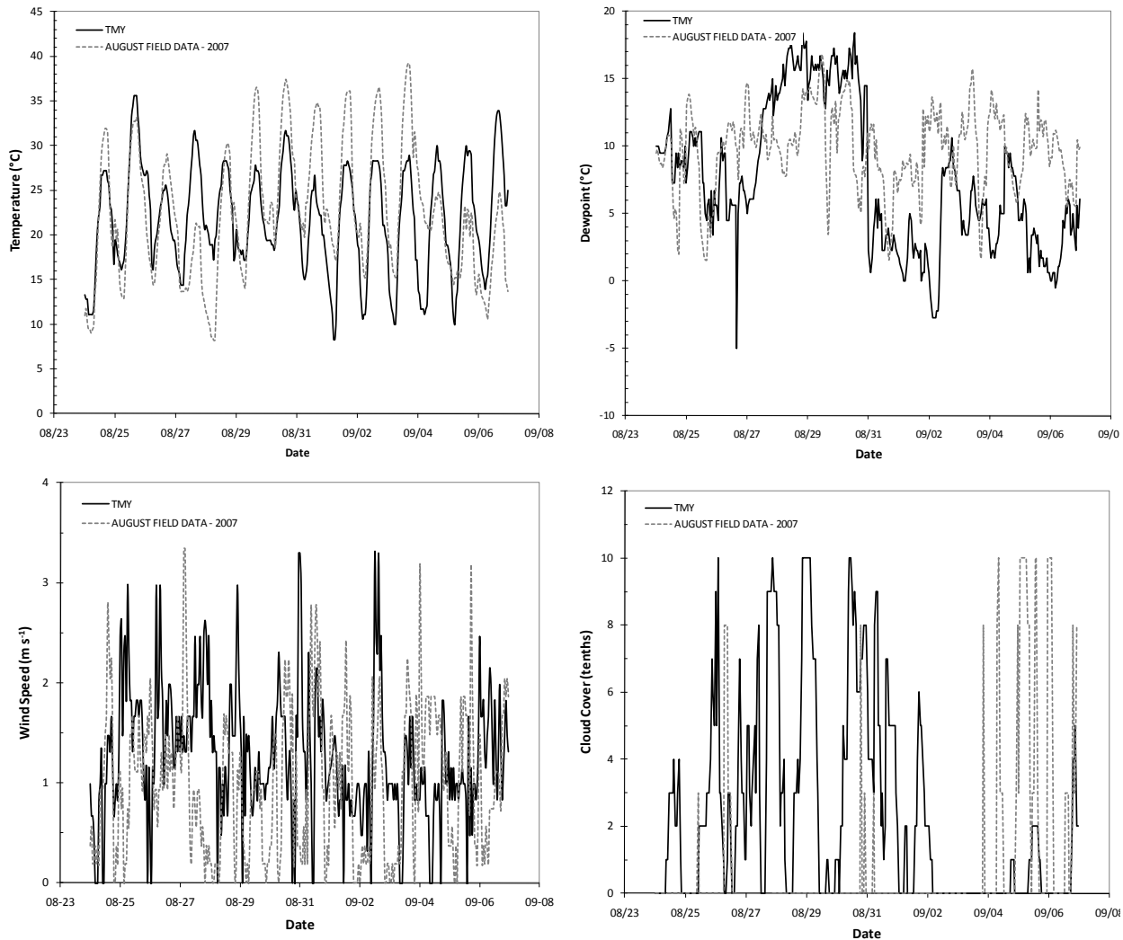
Figure 12-7. Plots of adjusted TMY in comparison with August 2007 field data. (Top left/right) Air temperature and dew point temperature (°C). (Bottom left/right) Wind speed (m s -1 ) and cloud cover (tenths). Adjustments are based on Table 12-3 .
