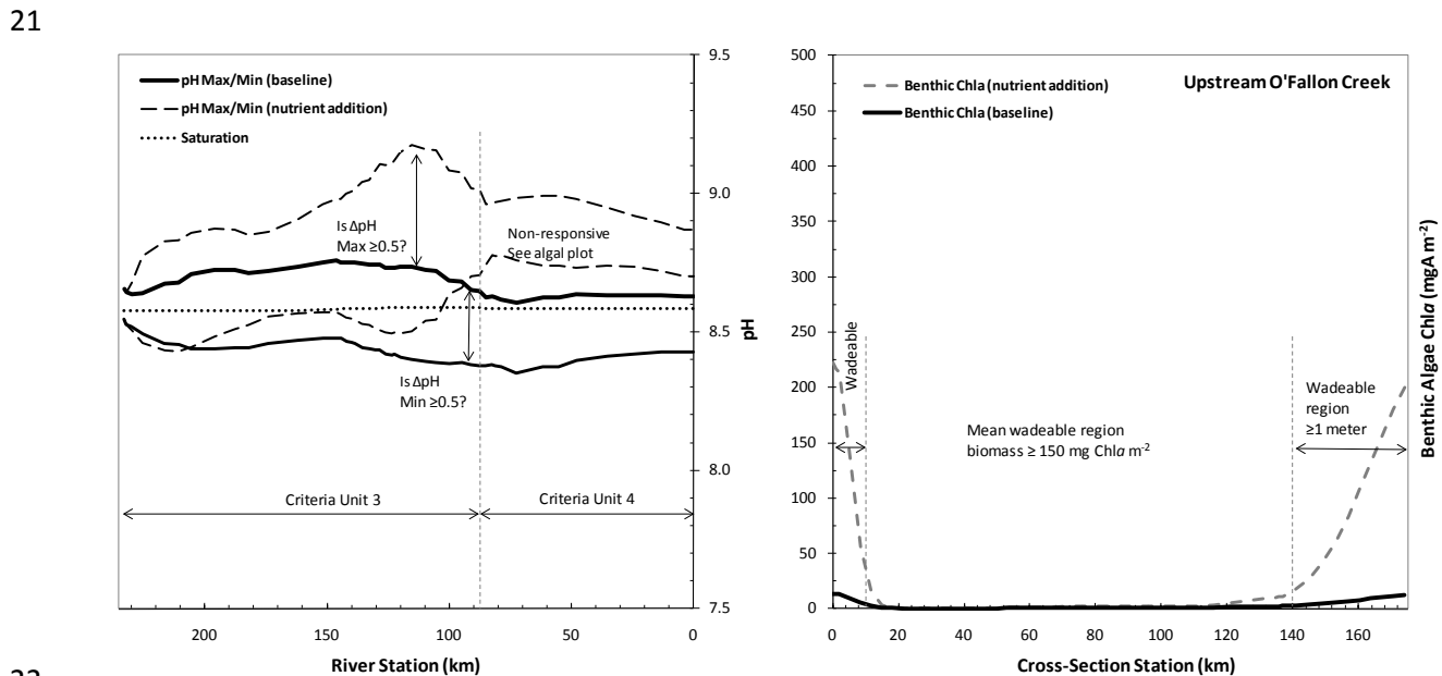
22 23 24 Figure 13-3. Example of a water quality endpoint determination. 25 (Left panel) Derivation of pH impairment using the differential between baseline and subsequent nutrient addition 26 Q2K runs. (Right panel) Same but for benthic algae, considering the wadeable region in AT2K.
