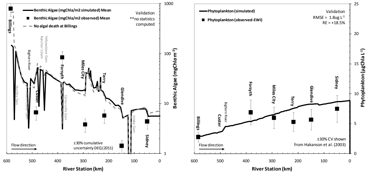
6 7 Figure 11-9. Algal simulations for the Yellowstone River during August 2000. 8 (Left panel) Simulated and observed benthic algae. (Right panel) Same but for phytoplankton. 9
