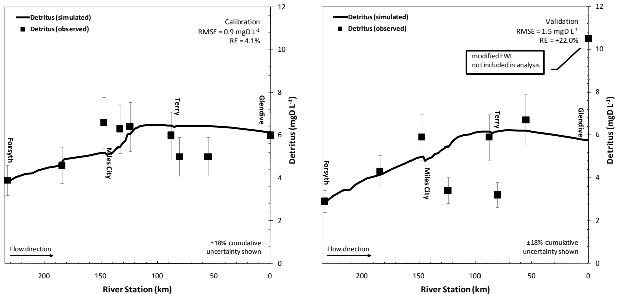
6 7 Figure 10-6. Detritus simulation for the lower Yellowstone River during 2007.
