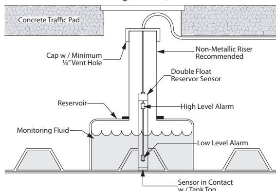
Figure 18-2 For Tanks Larger than 1,000 Gallons
