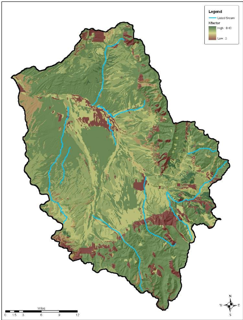
Figure 2-2. USLE K-factor for the Lower Gallatin River Watershed.
