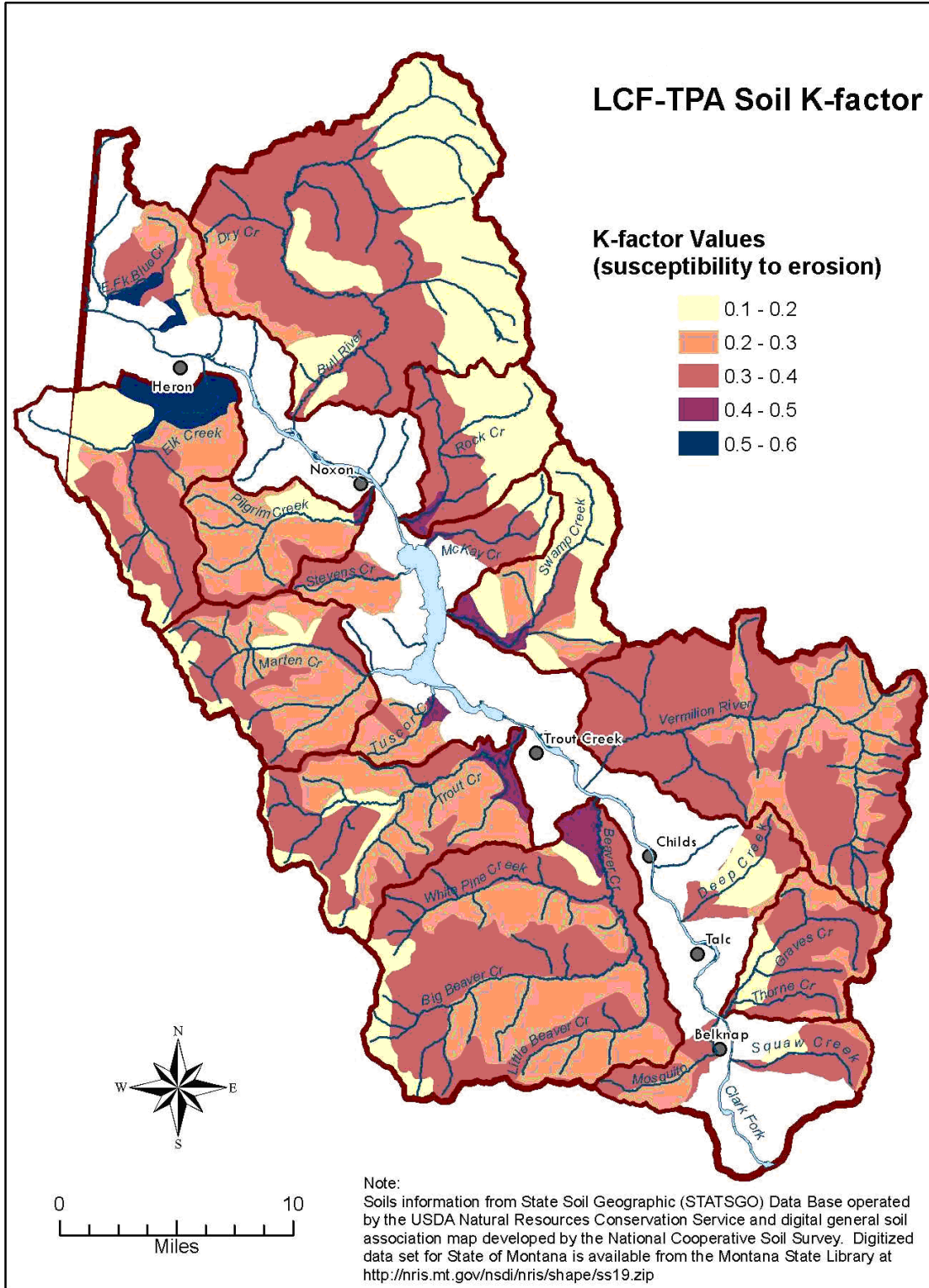
Figure A-4. K-Factors
