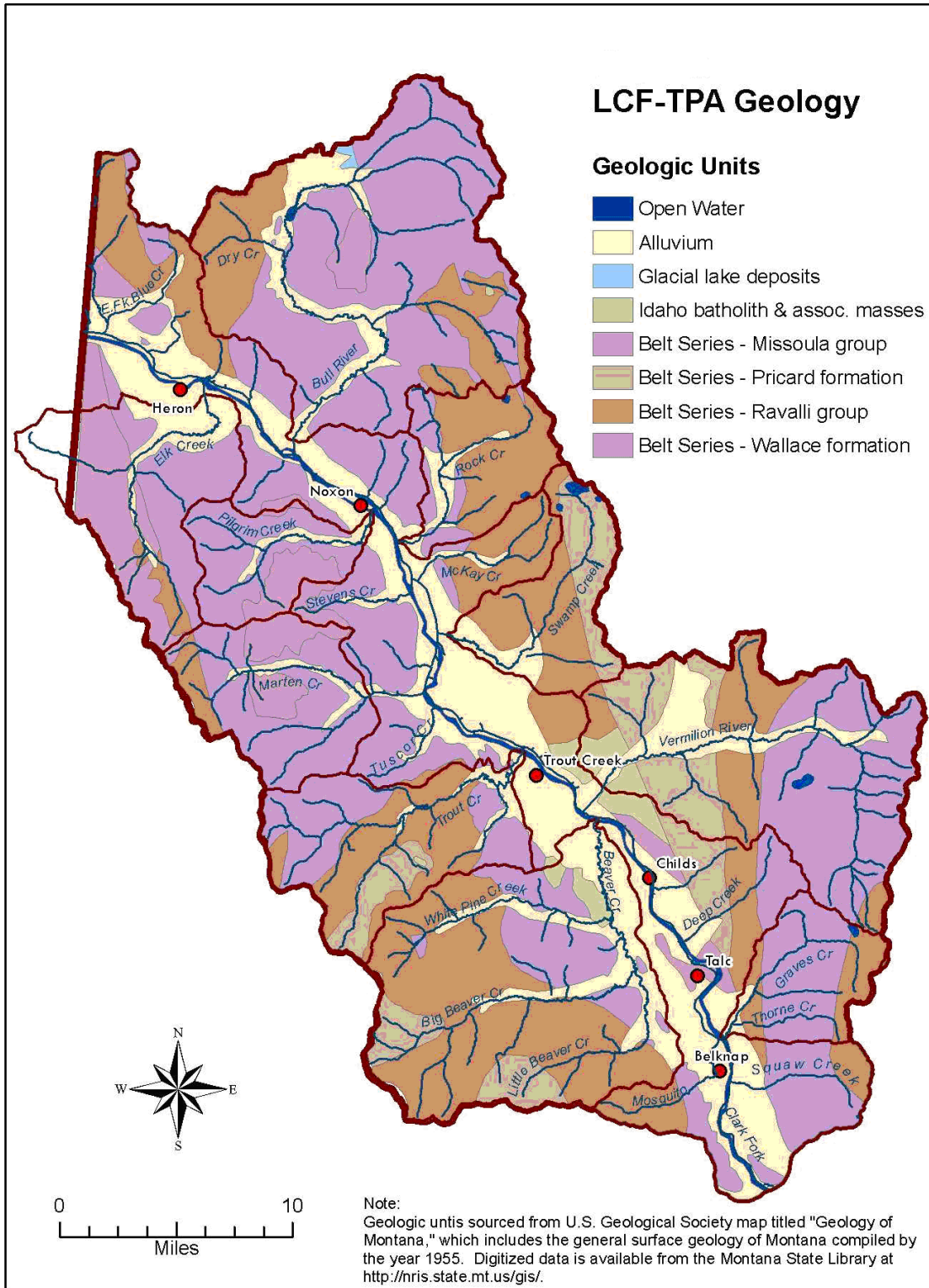
Figure A-3. Geology
