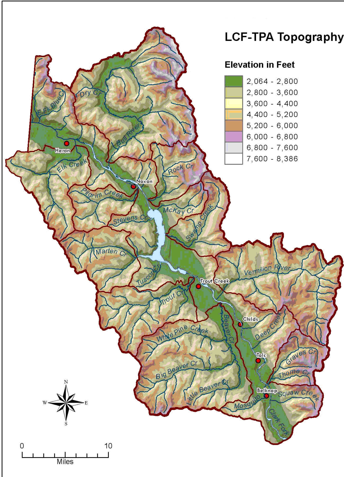
Figure A-2. Topography
