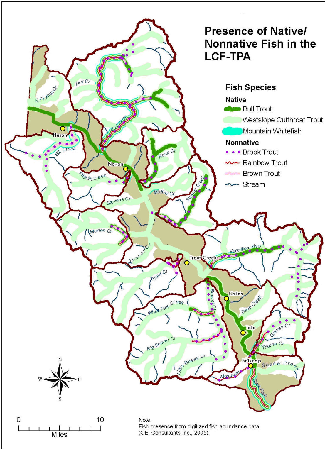
Figure A-6. Fish Species Distribution
