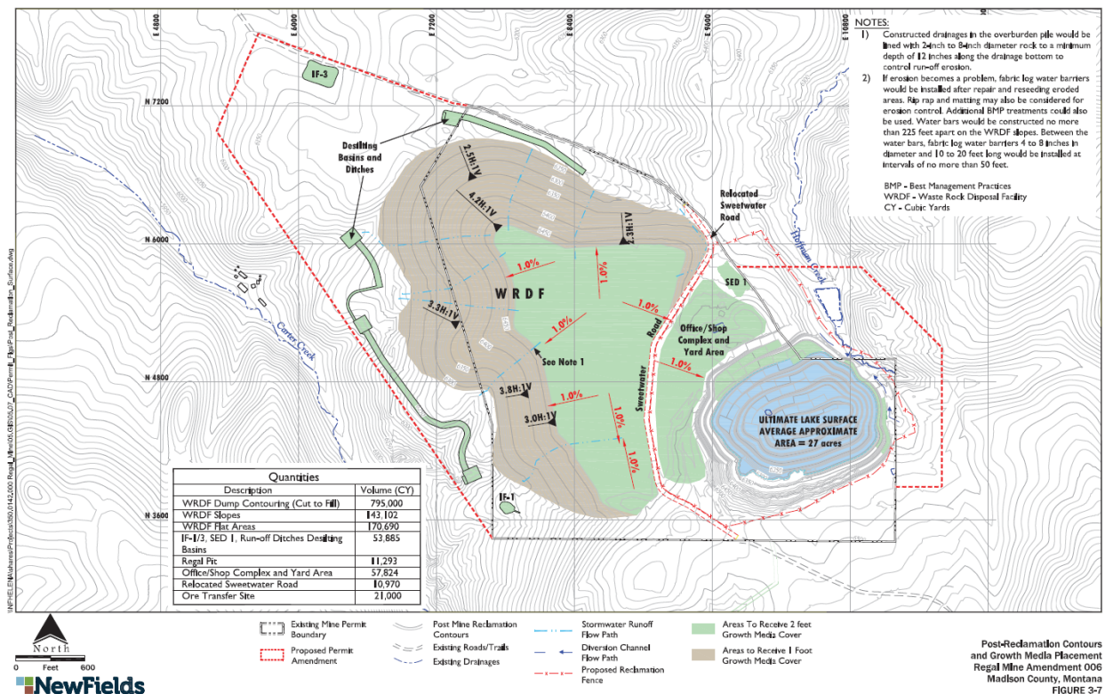
Figure 3.11-2 Final Reclamation Contours and Growth Media Placement
