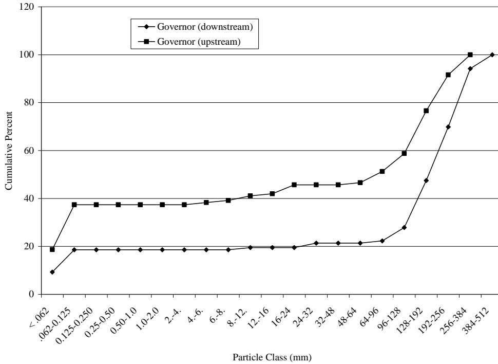
Figure 5-4: Cumulative percent frequency of particles sampled in pebble counts on the Governor Creek in 1999 collected by USFS.
