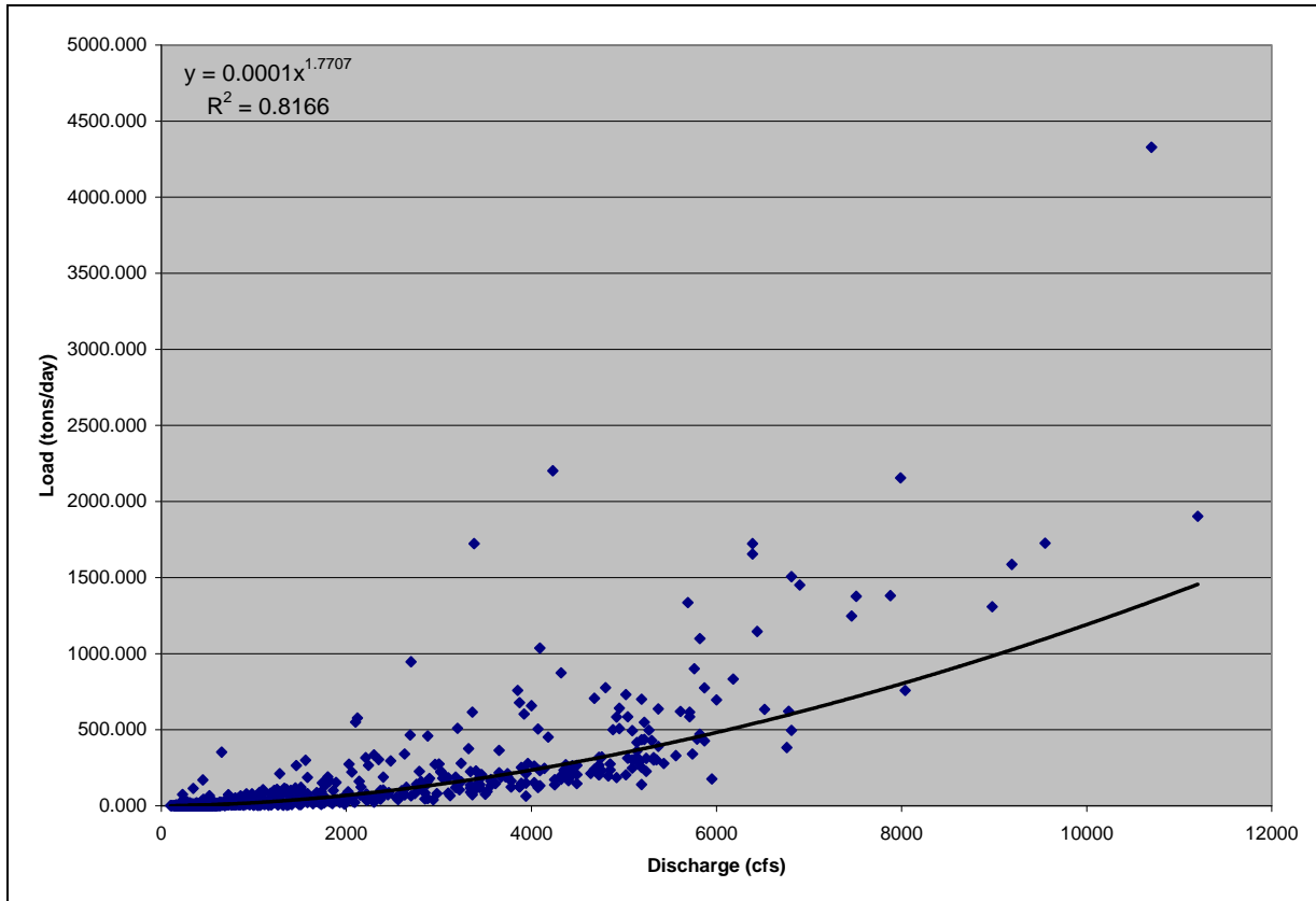
Figure H-1. Sediment Rating Curve for the Big Hole River
