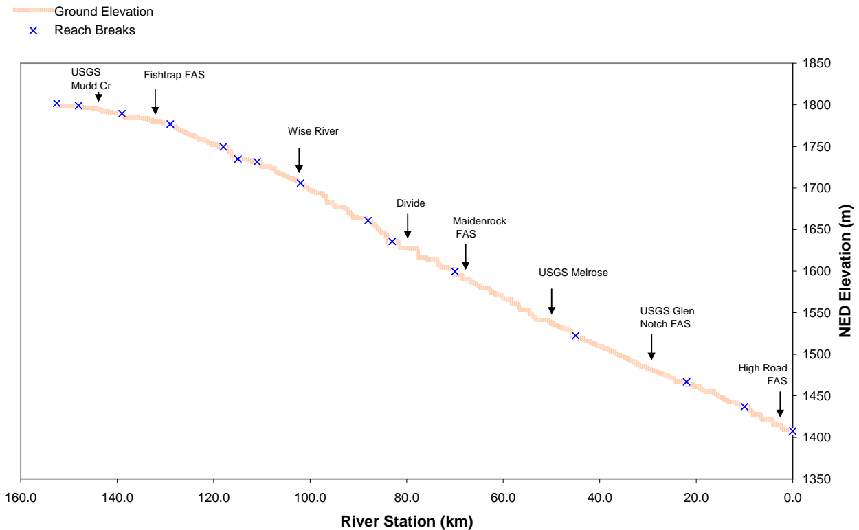
Figure 9. Unique reaches defined for model parameterization of hydraulics. Elevation data taken from USGS National Elevation Dataset (NED) 30-m grid.
