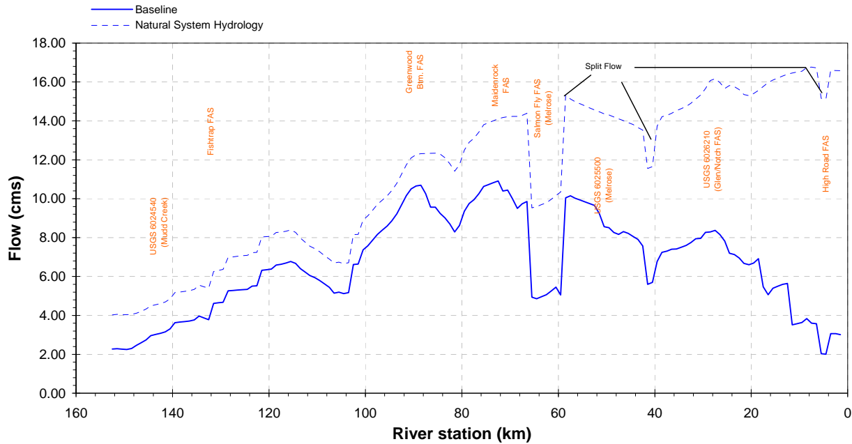
Figure 18. Longitudinal profile of discharge in the watershed as part of the water use scenario. The 1.75 m 3 /s headwater increase is included in this approximation along with removal of all diversions in the study area.
