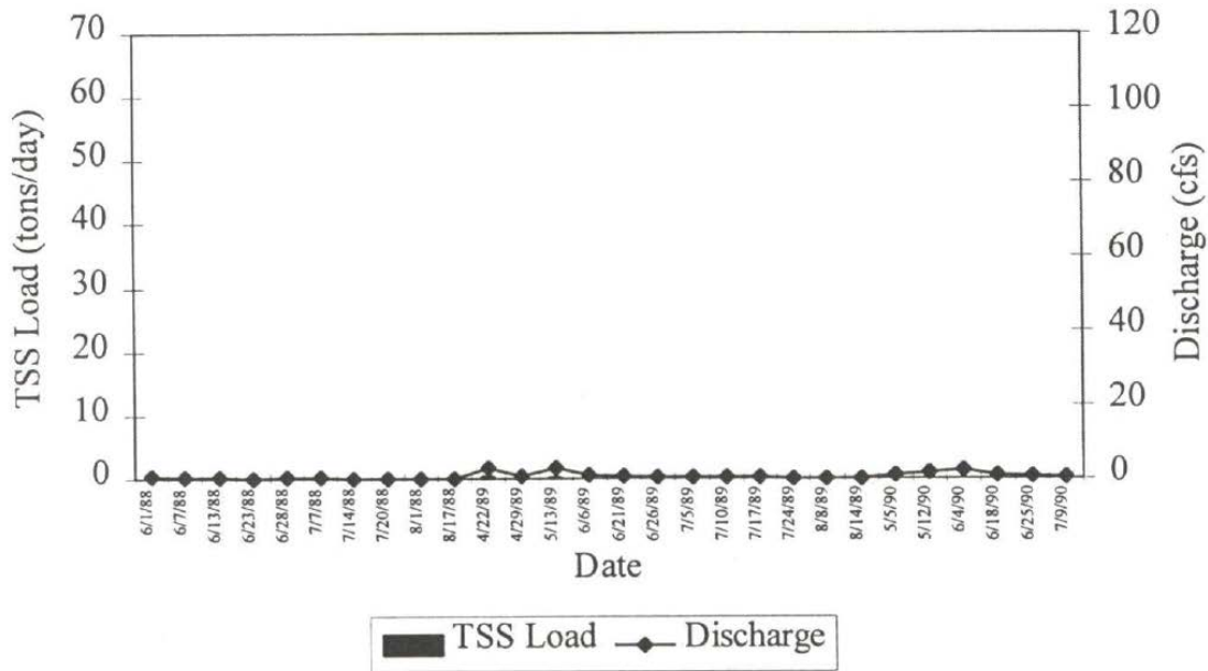
Figure 6b. Daily TSS load and discharge per sampling date at Carl Creek water sampling site
