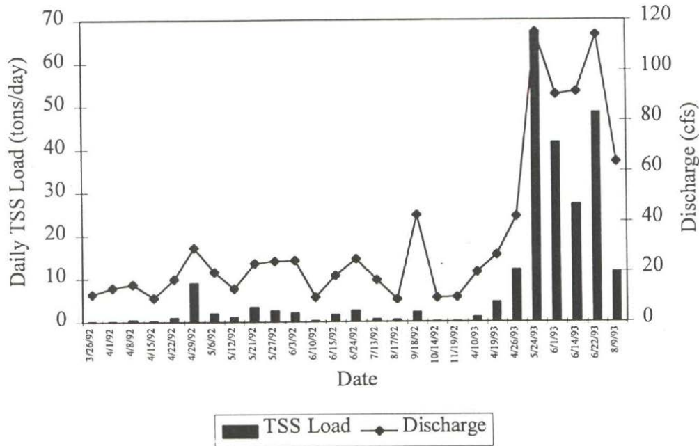
Figure 1b. Daily TSS load and discharge per sampling date for above Montana Ditch water sampling site
