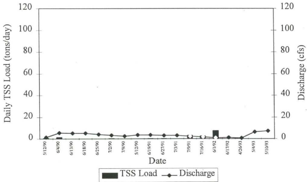
Figure 4b. Daily TSS load and discharge per sampling date at Cabin Gulch water sampling site
