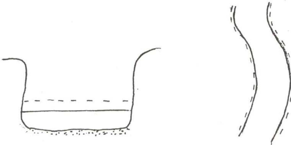
Figure 1d. Stream Type F4, cross-sectional and aerial view. This stream type is totally entrenched (little or no floodplain) with a predominately gravel substrate. F4 channels are characterized by very high width/depth ratio, slight to moderate sinuosity, and moderate slope. Because of deep entrenchment of the channel, high flows exert high boundary stress on banks resulting in excessive erosion. The high width/depth ratio results in poor sediment on the streambed. Since the banks are nearly vertical, establishment of stabilizing vegetation to reduce erodibility is difficult.
