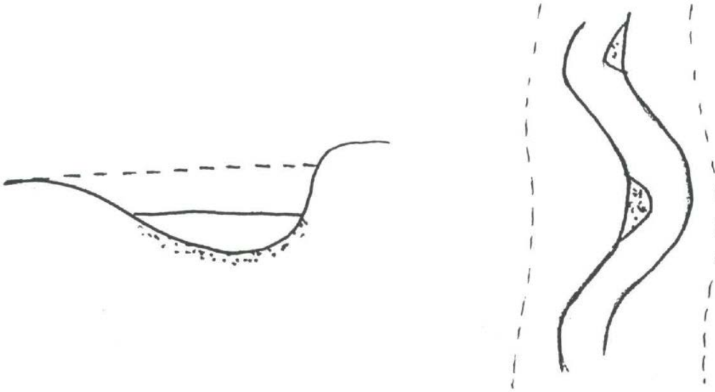
Figure 3d. Stream Type C4, cross-sectional and aerial view. This channel type is slightly entrenched with a well developed floodplain and a gravel substrate. Sinuosities range from high to moderate and width/depth ratios are moderate. Slopes are generally gentle. These channels are characterized by alternating riffle and pool habitat types. With proper riparian management, these are stable stream types. Although high flows exert stress against outer channel bends, flows greater than bankfull spread out over the adjacent floodplain.
