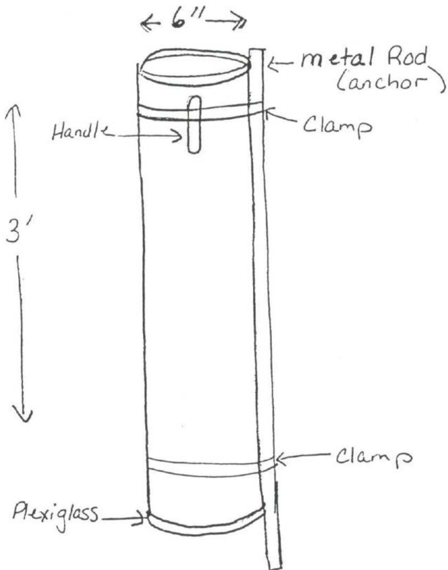
Figure 1F. Diagram of PVC pipe for photographing substrate (as described by C. Harnish). Twelve pictures per percent fines grid are needed to get a complete photographic series of the grid.
