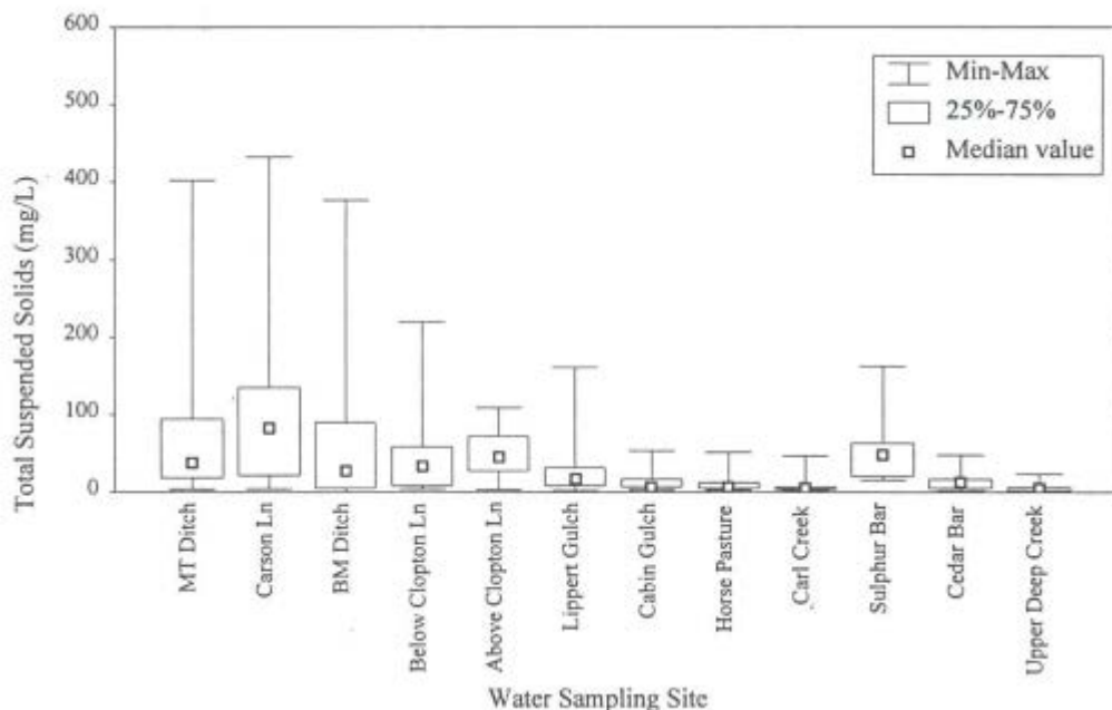
Figure 8. Total suspended solids concentration at each water sampling site.
