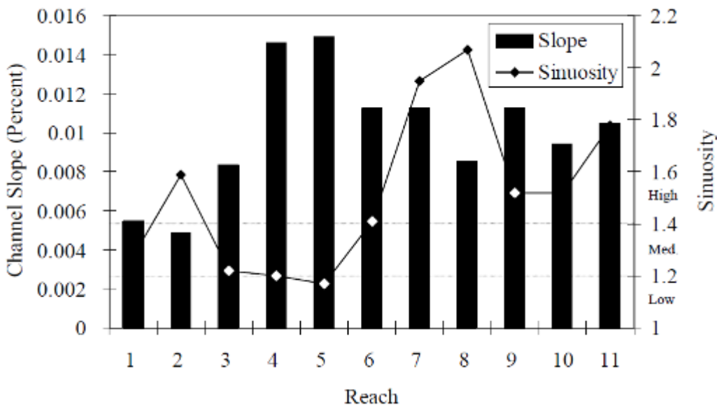
Figure 11. Channel slope and sinuosity by reach. Horizontal lines designate boundaries for low, medium and high sinuosity ratings (Rosgen 1994).
