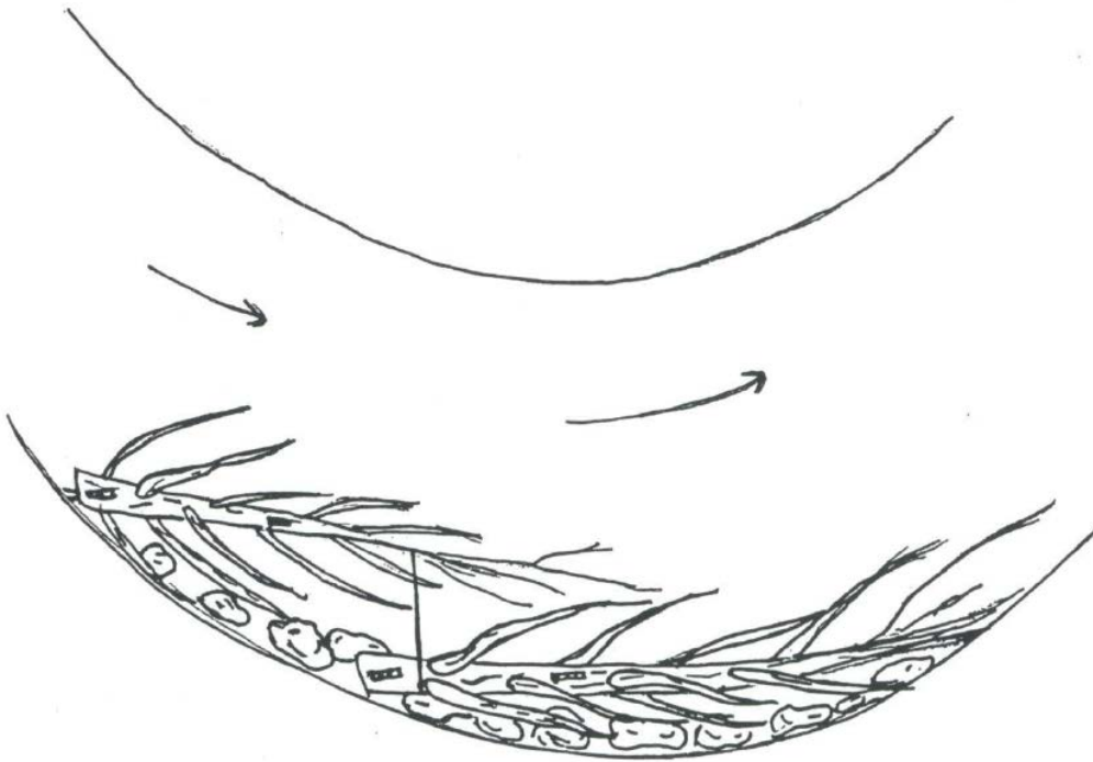
Figure 22. Diagram of juniper revetment for stabilizing outer meander bend
