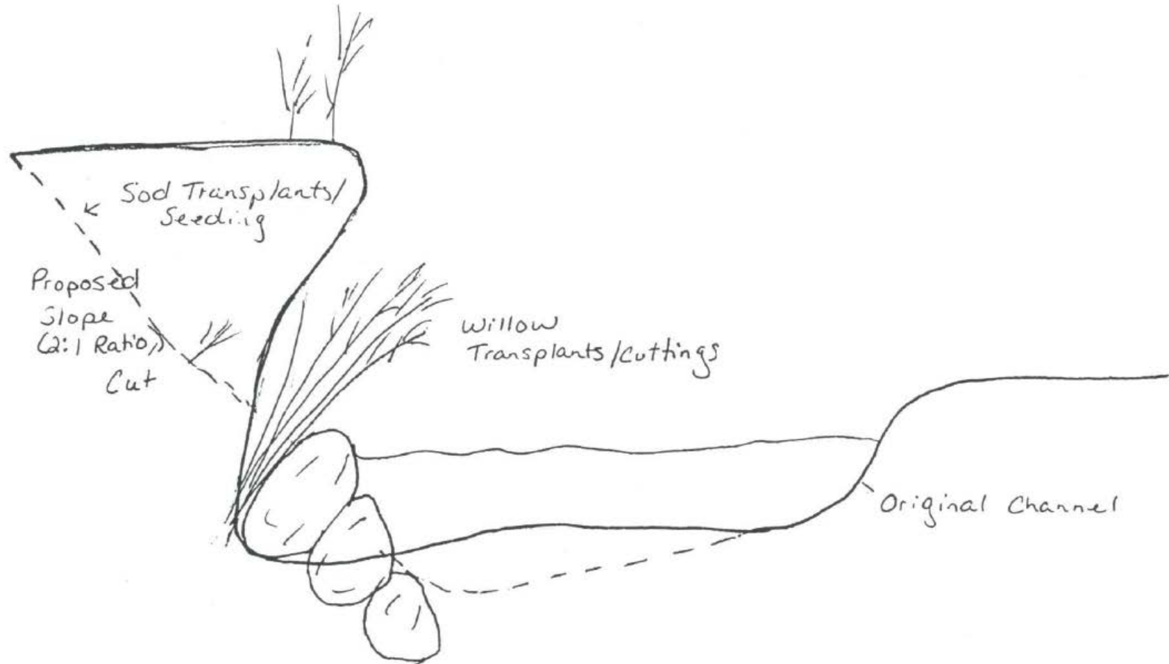
Figure 1e. Cross-sectional view of native material revetment for outside bend of incised streambank (alteration of F4 and G4 channel types to a C4 channel type).
