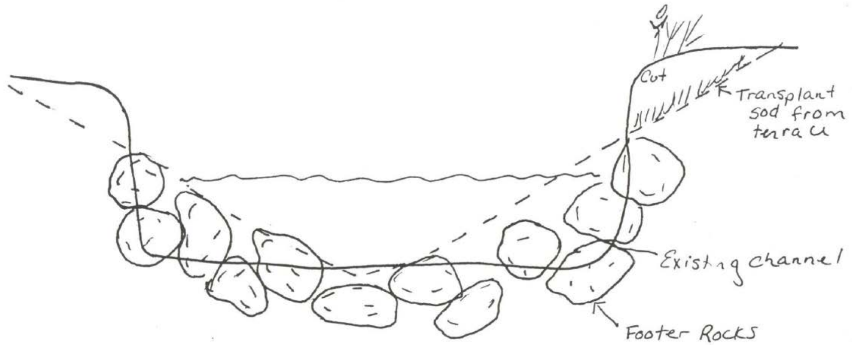
Figure 4e. Cross-section showing conversion of an unstable F4 channel type to a more stable B4 channel type. Spacing of weirs at 4 to 5 times bankfull width.
