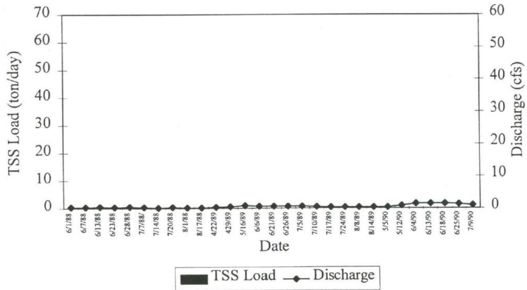
Figure 8b. Daily TSS load and discharge per sampling date at Cedar Bar water sampling site
