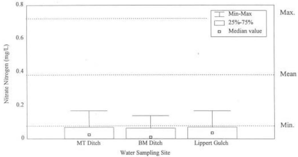
Figure 5. Nitrate-nitrogen per water sampling site. Horizontal lines represent minimum, mean, and maximum concentrations measured on Montana Valley and Foothill Prairies reference streams (Bahls et al. 1992).
