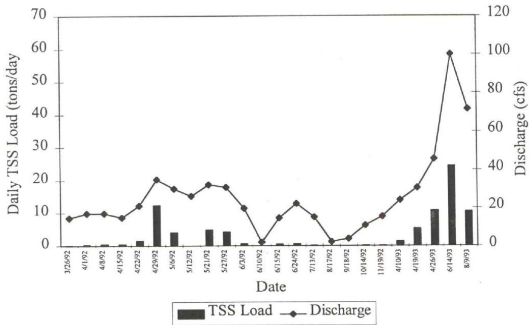
Figure 2b. Daily TSS load and discharge pre sampling date for above Broadwater-Missouri ditch water sampling site
