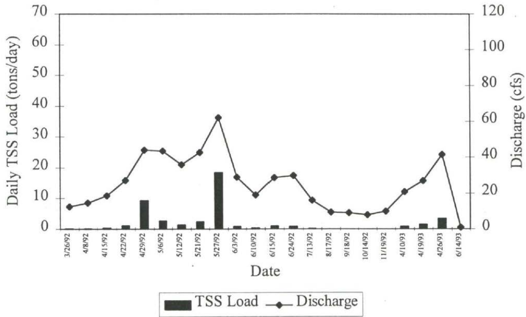
Figure 3b. Daily TSS load and discharge per sampling date at Lippert Gulch water sampling site
