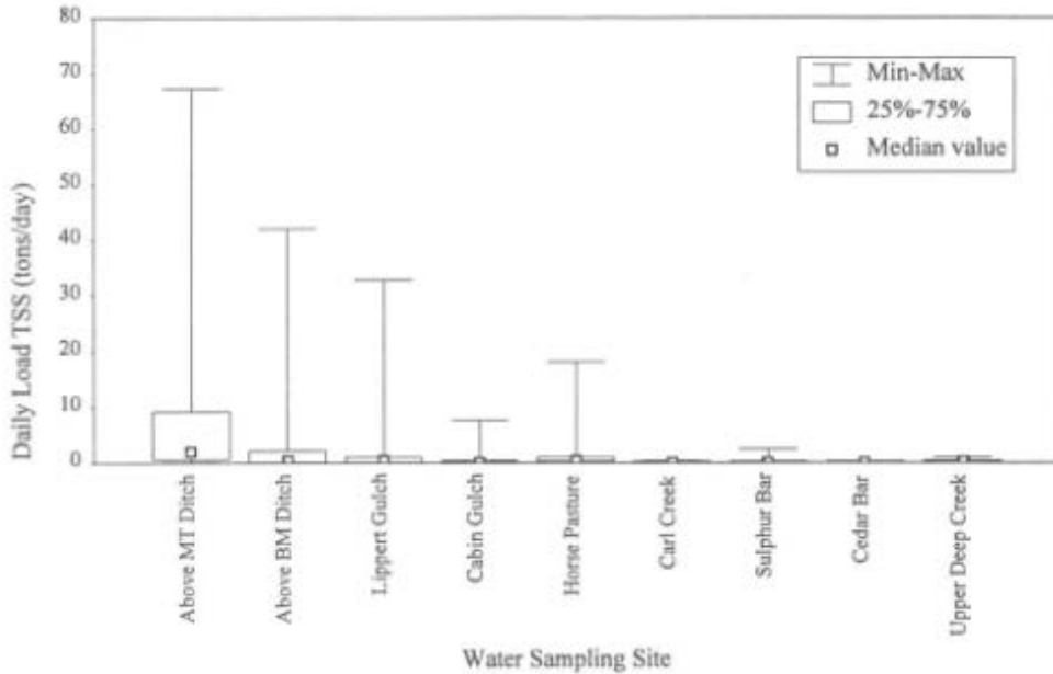
Figure 9. Daily load of total suspended solids per water sampling site.
