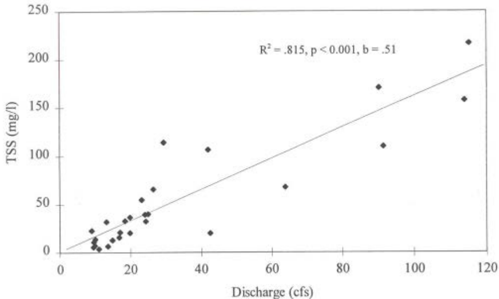
Figure 10. Relationship between TSS concentration and discharge at Montana Ditch.
