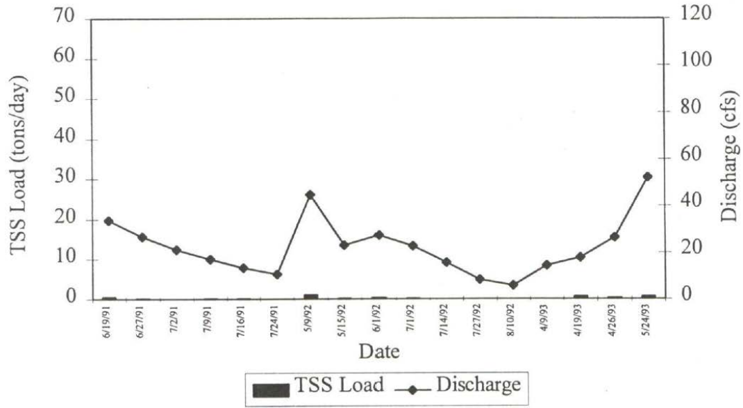
Figure 9b. Daily TSS load and discharge per sampling date at Upper Deep Creek water sampling site
