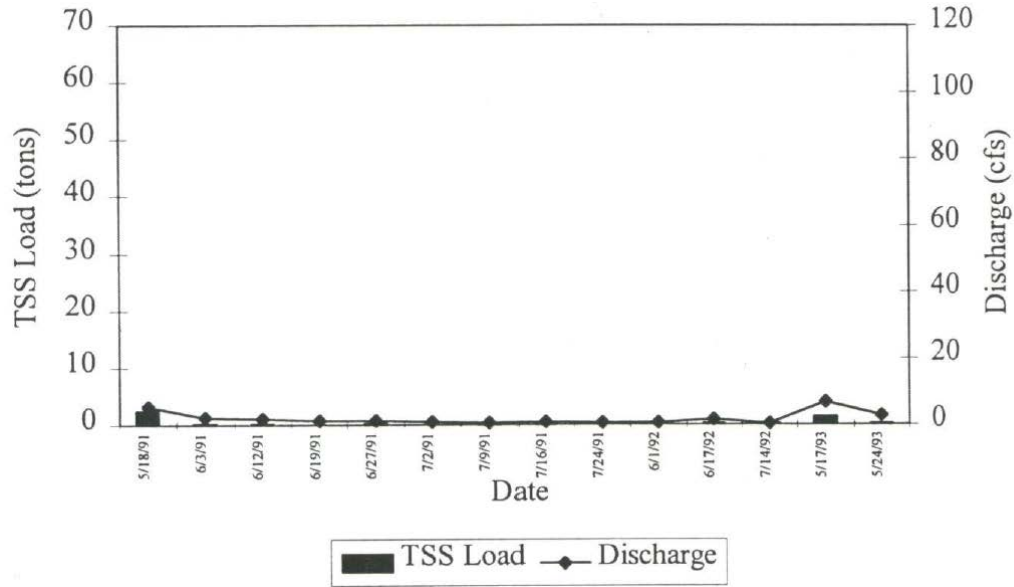
Figure 7b. Daily TSS load and discharge per water sampling date at Sulphur Bar water sampling site
