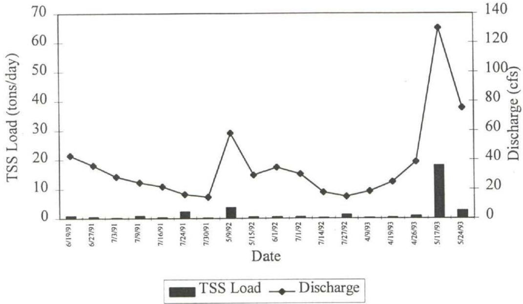
Figure 5b. Daily TSS load and discharge per sampling date at Horse pasture water sampling site
