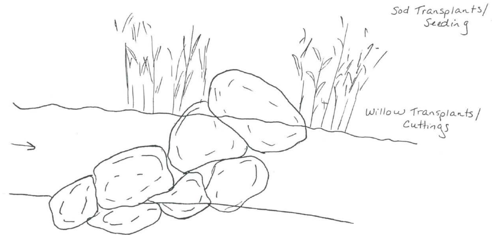
Figure 3e. Side view of native material revetment for erosive, outside channel bend (alteration of F4 and G4 channel types to a C4 channel type).
