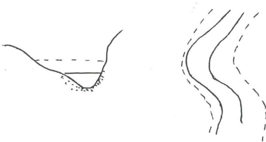
Figure 4d. Stream Type G4, cross-sectional and aerial views. These are “gully streams” with a predominately gravel streambeds. They are highly entrenched and characterized by low width/depth ratio and low to moderate sinuosity.
