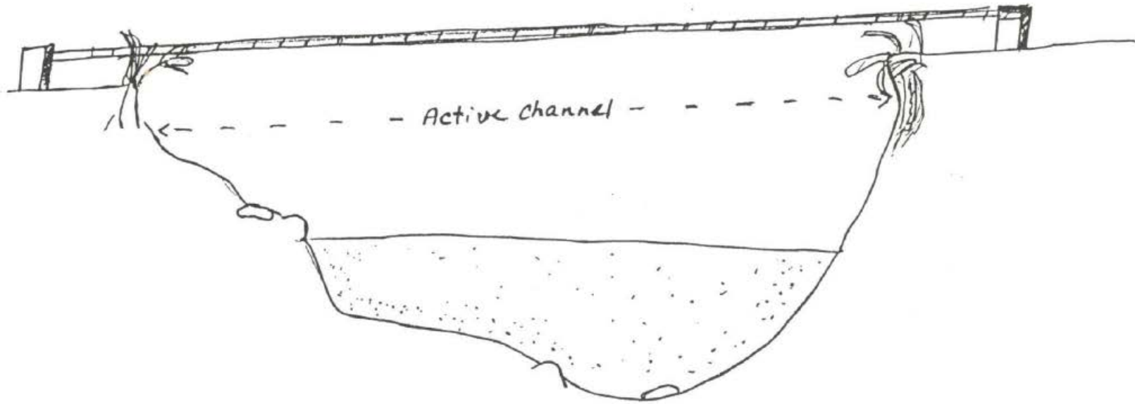
Figure 2f. Diagram of channel cross-section.
