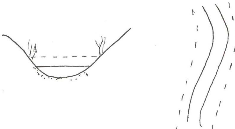
Figure 2d. Stream Type B4c, cross-sectional and aerial view. This stream type is moderately entrenched with a gravel streambed. Width/depth ratio is moderate and slope is gentle. This is a generally a stable stream type with vegetated stream banks. B4 channel types do not generally accumulate sediment. These channel types are often riffle dominated and often do not provide much high quality fish habitat.
