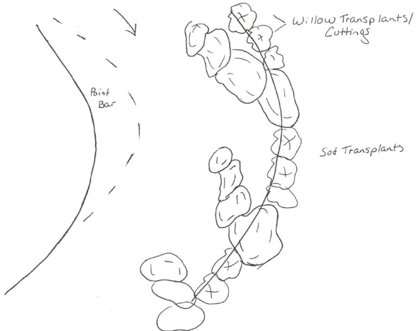
Figure 2e. Plan-view of native material revetment on outside bend of erosive bank (alteration of F4 and G4 channel types to a C4 channel type).
