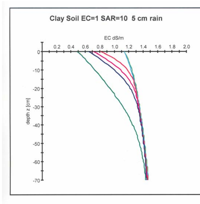
Figure 31. Predicted relationship of EC with depth and quantity of rain infiltrated into the clay soil. The initial condition was EC=1.0 dS/m and SAR 10. Each curve represents addition of 1 cm of rain.
