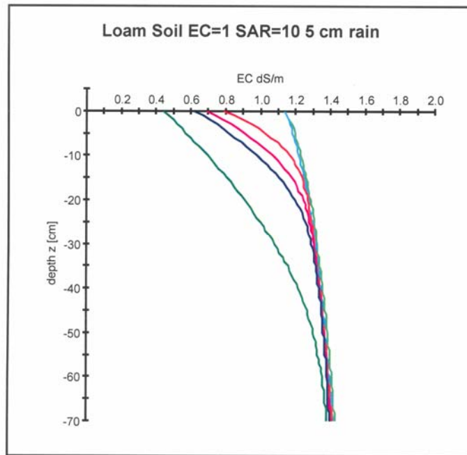
Figure 29. Predicted relationship of EC with depth and quantity of rain infiltrated for Glendive loam soil. The initial condition was EC=1.0 dS/m and SAR 10. Each curve represents addition of 1 cm of rain.
