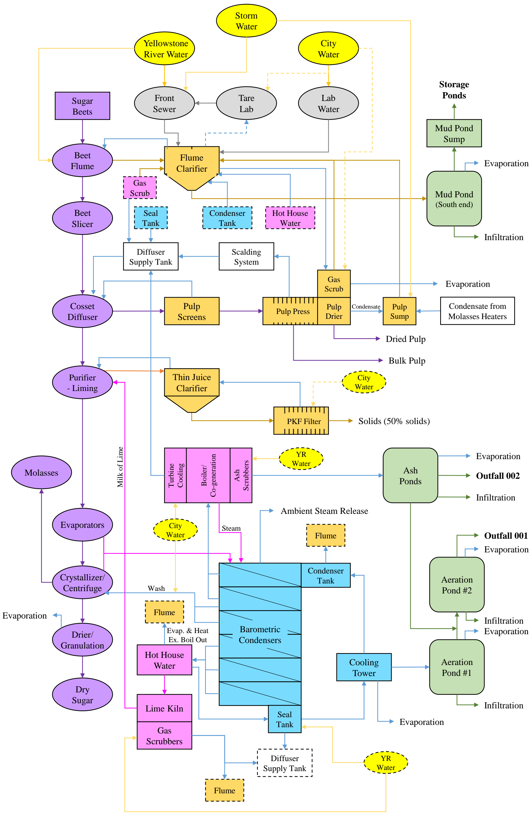
WESTERN SUGAR FLOW REDUCTION REPORT WATER FLOW DIAGRAM – EXISTING CONDITIONS
