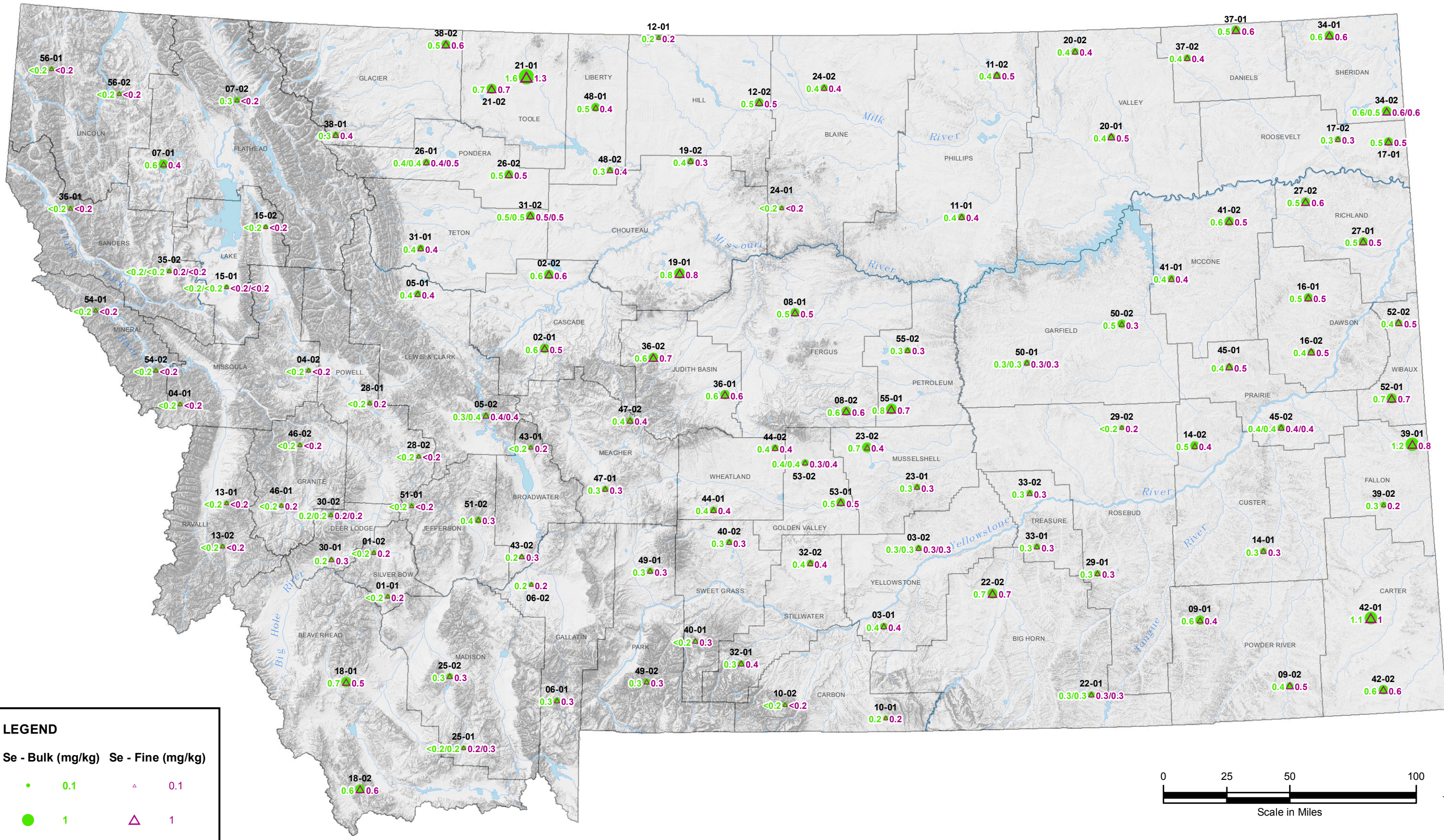
BACKGROUND CONCENTRATIONS OF INORGANIC CONSTITUENTS IN MONTANA SURFACE SOILS SELENIUM CONCENTRATIONS (mg/kg) BULK AND FINE FRACTION SAMPLES FIGURE C-16
