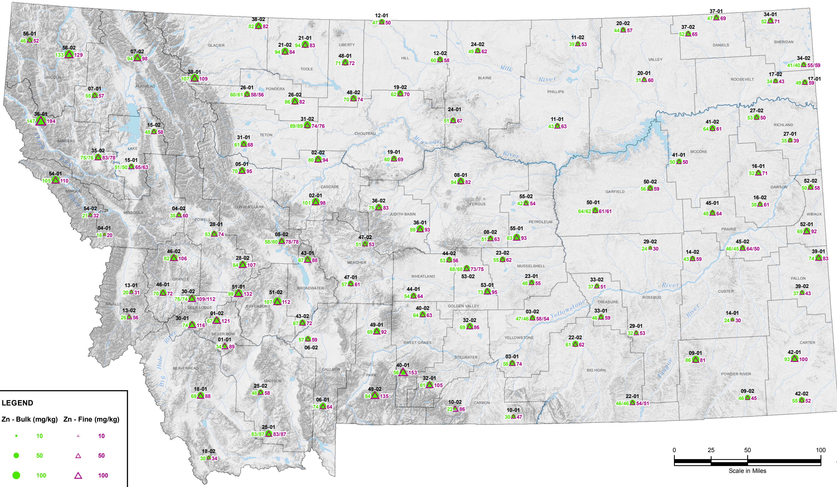
BACKGROUND CONCENTRATIONS OF INORGANIC CONSTITUENTS IN MONTANA SURFACE SOILS ZINC CONCENTRATIONS (mg/kg) BULK AND FINE FRACTION SAMPLES FIGURE C-20
