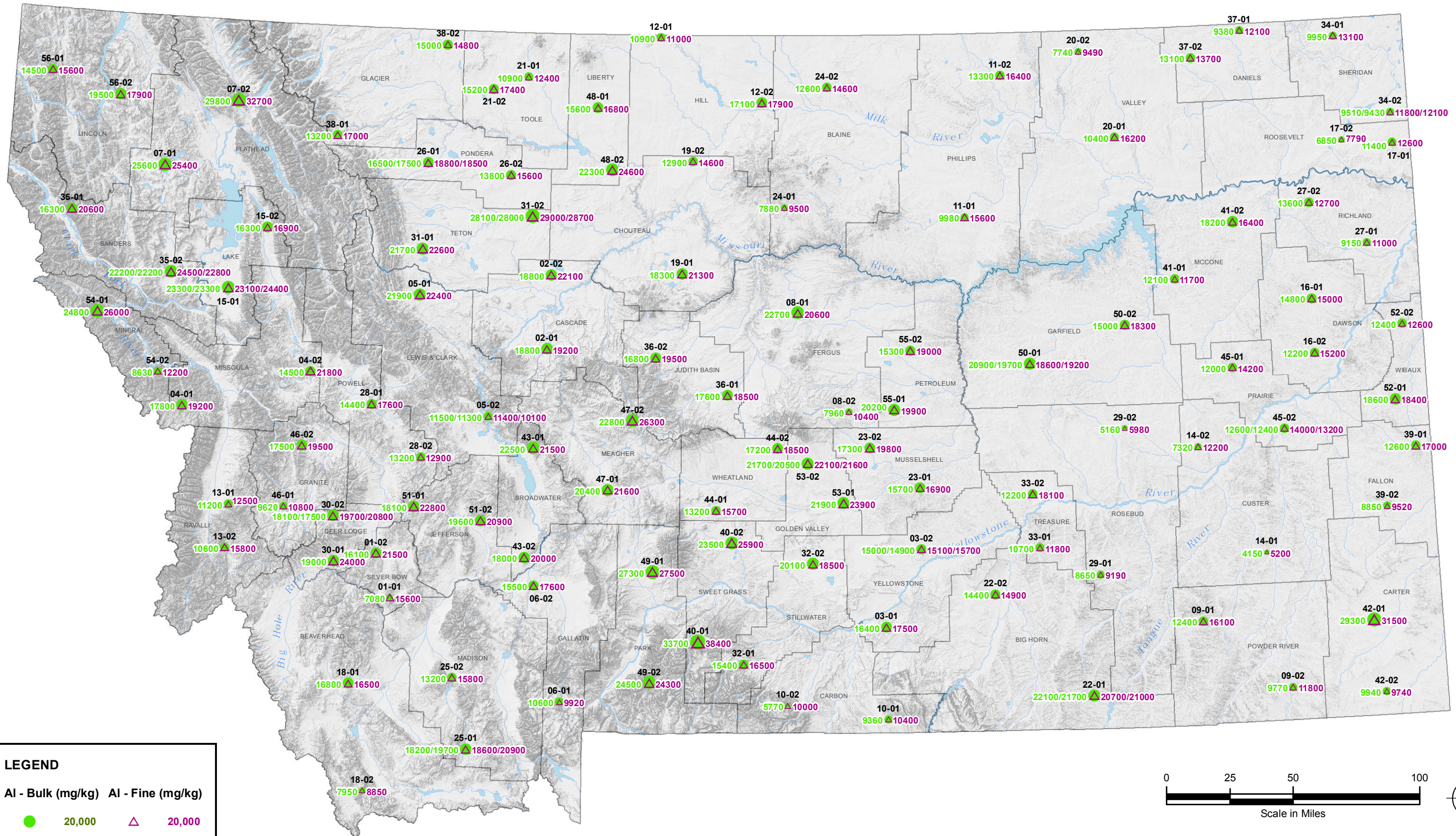
BACKGROUND CONCENTRATIONS OF INORGANIC CONSTITUENTS IN MONTANA SURFACE SOILS ALUMINUM CONCENTRATIONS (mg/kg) BULK AND FINE FRACTION SAMPLES FIGURE C-1
