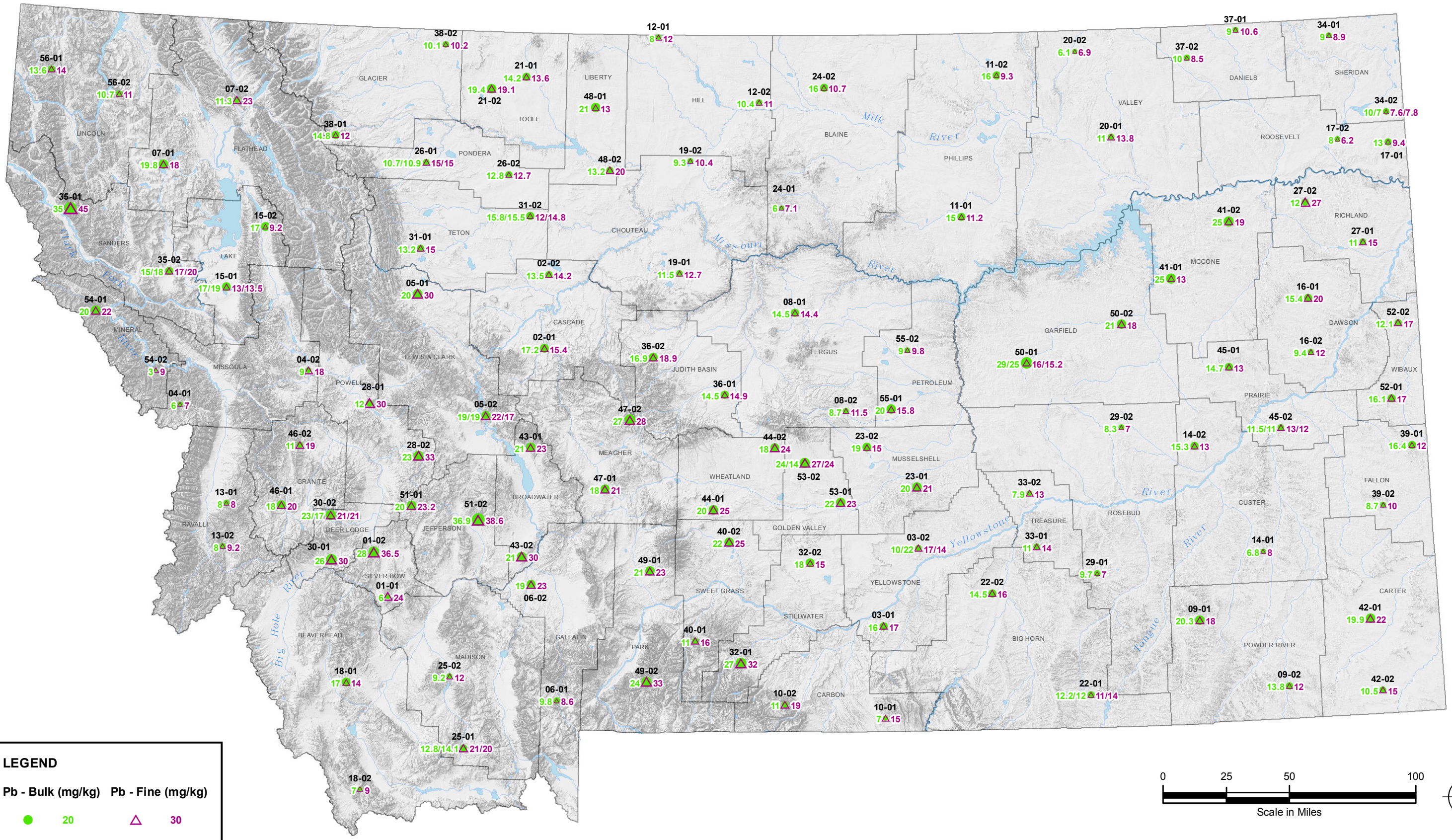
BACKGROUND CONCENTRATIONS OF INORGANIC CONSTITUENTS IN MONTANA SURFACE SOILS LEAD CONCENTRATIONS (mg/kg) BULK AND FINE FRACTION SAMPLES FIGURE C-12
