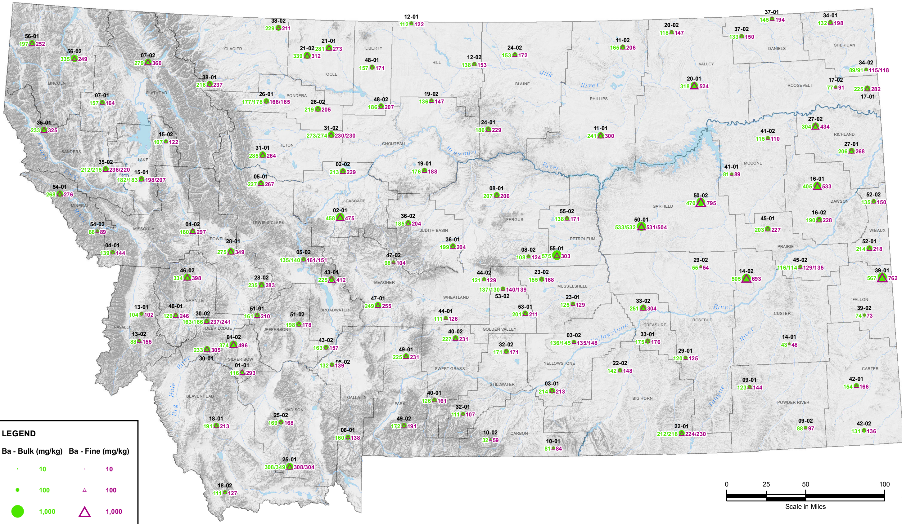
BACKGROUND CONCENTRATIONS OF INORGANIC CONSTITUENTS IN MONTANA SURFACE SOILS BARIUM CONCENTRATIONS (mg/kg) BULK AND FINE FRACTION SAMPLES FIGURE C-4
