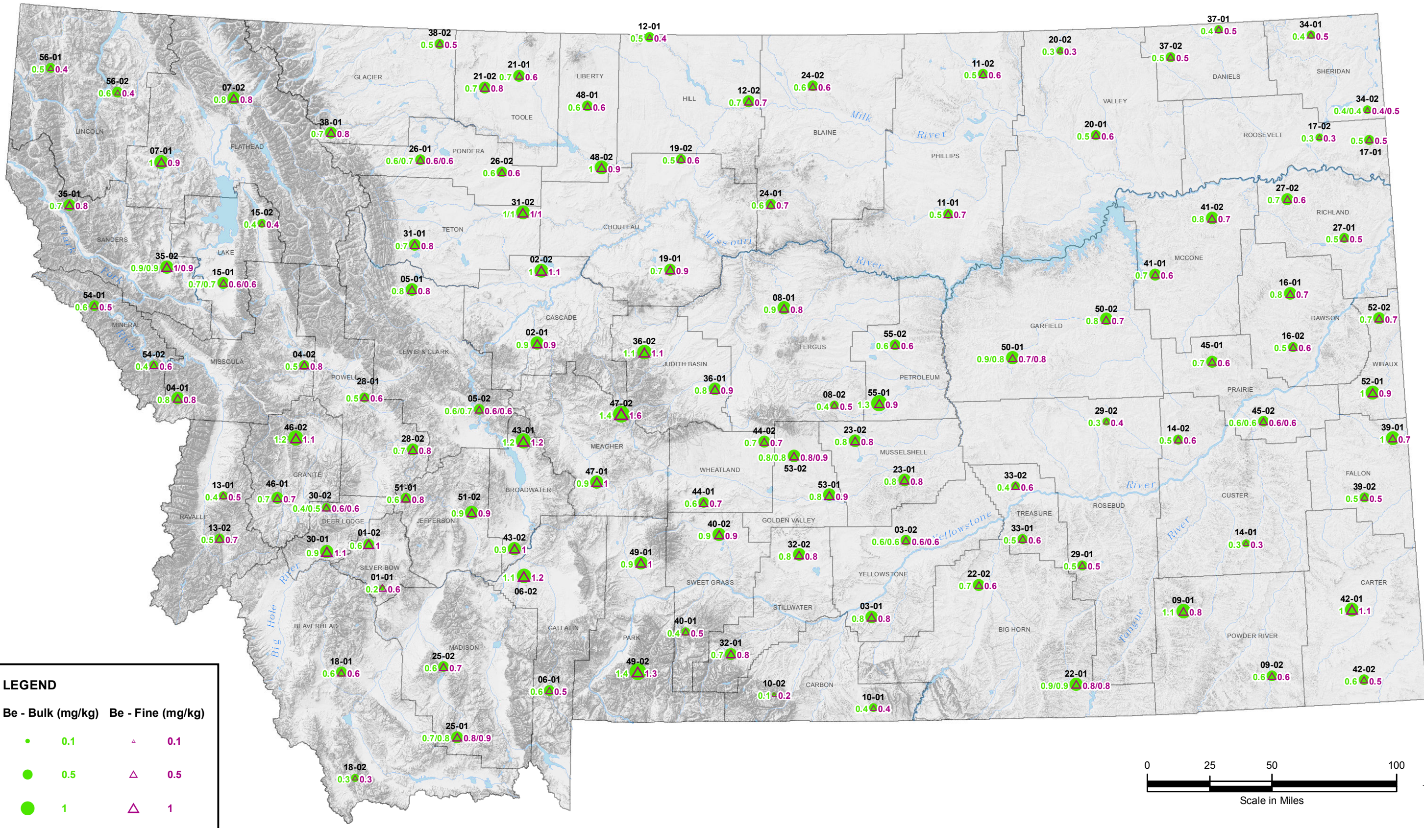
BACKGROUND CONCENTRATIONS OF INORGANIC CONSTITUENTS IN MONTANA SURFACE SOILS BERYLLIUM CONCENTRATIONS (mg/kg) BULK AND FINE FRACTION SAMPLES FIGURE C-5
