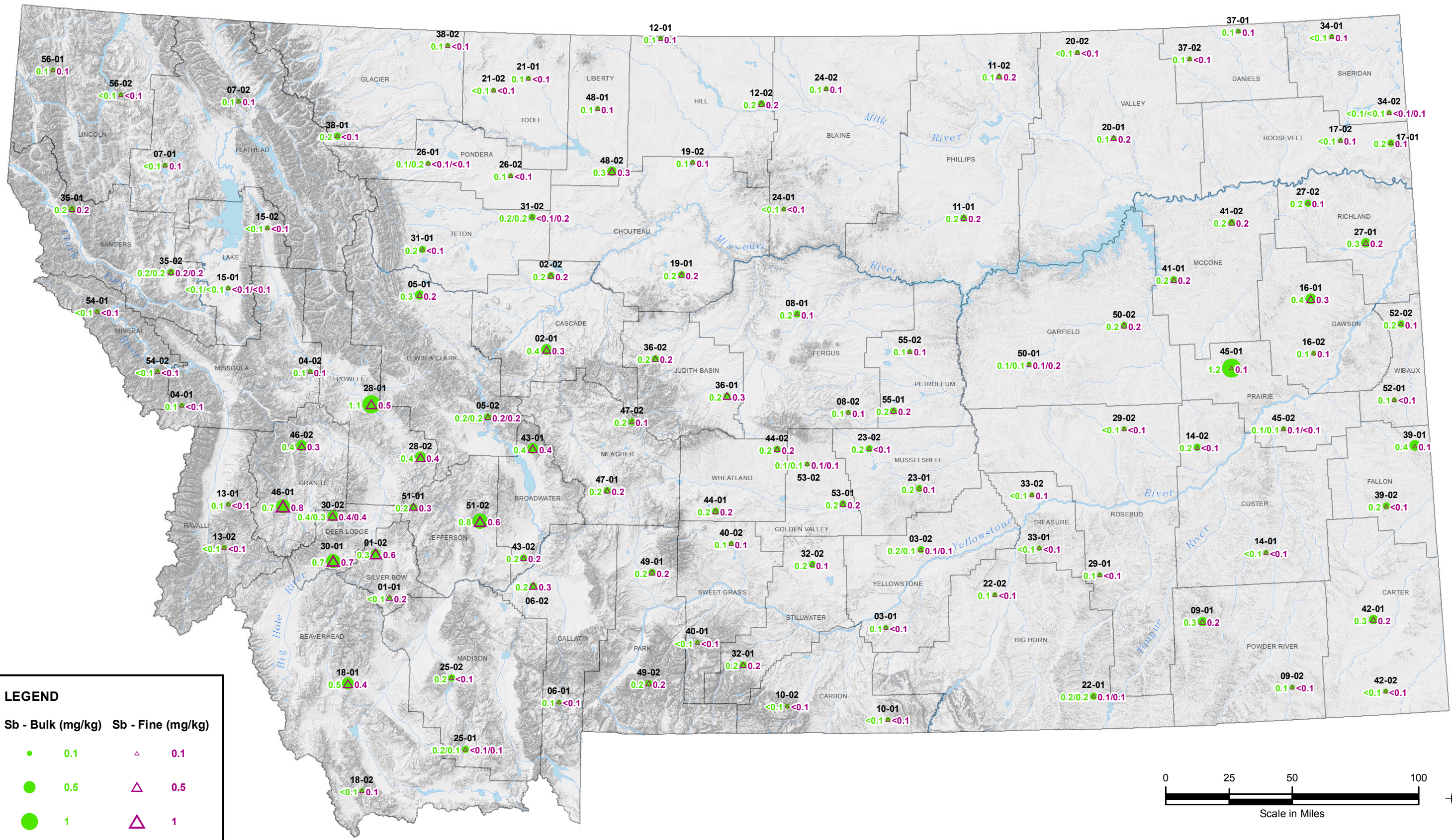
BACKGROUND CONCENTRATIONS OF INORGANIC CONSTITUENTS IN MONTANA SURFACE SOILS ANTIMONY CONCENTRATIONS (mg/kg) BULK AND FINE FRACTION SAMPLES FIGURE C-2
