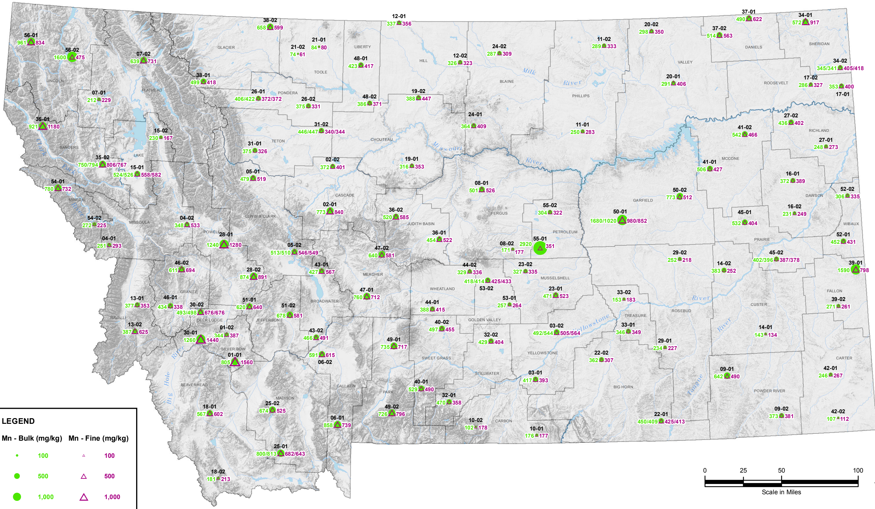
BACKGROUND CONCENTRATIONS OF INORGANIC CONSTITUENTS IN MONTANA SURFACE SOILS MANGANESE CONCENTRATIONS (mg/kg) BULK AND FINE FRACTION SAMPLES FIGURE C-13
