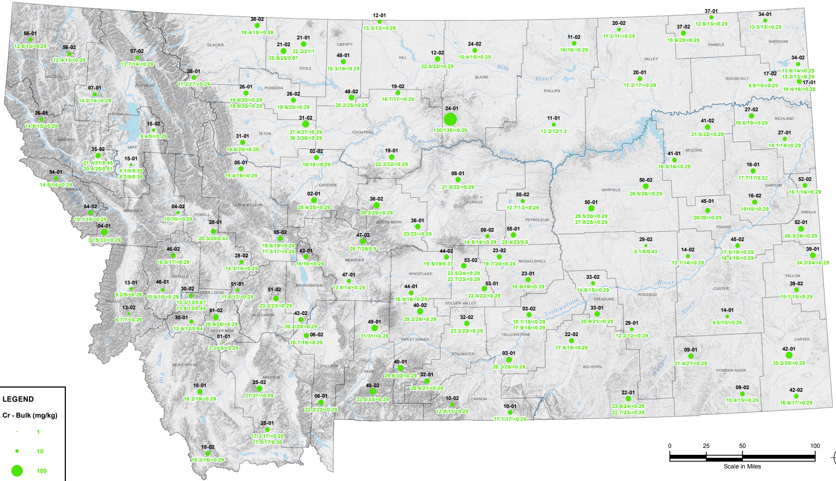
BACKGROUND CONCENTRATIONS OF INORGANIC CONSTITUENTS IN MONTANA SURFACE SOILS
