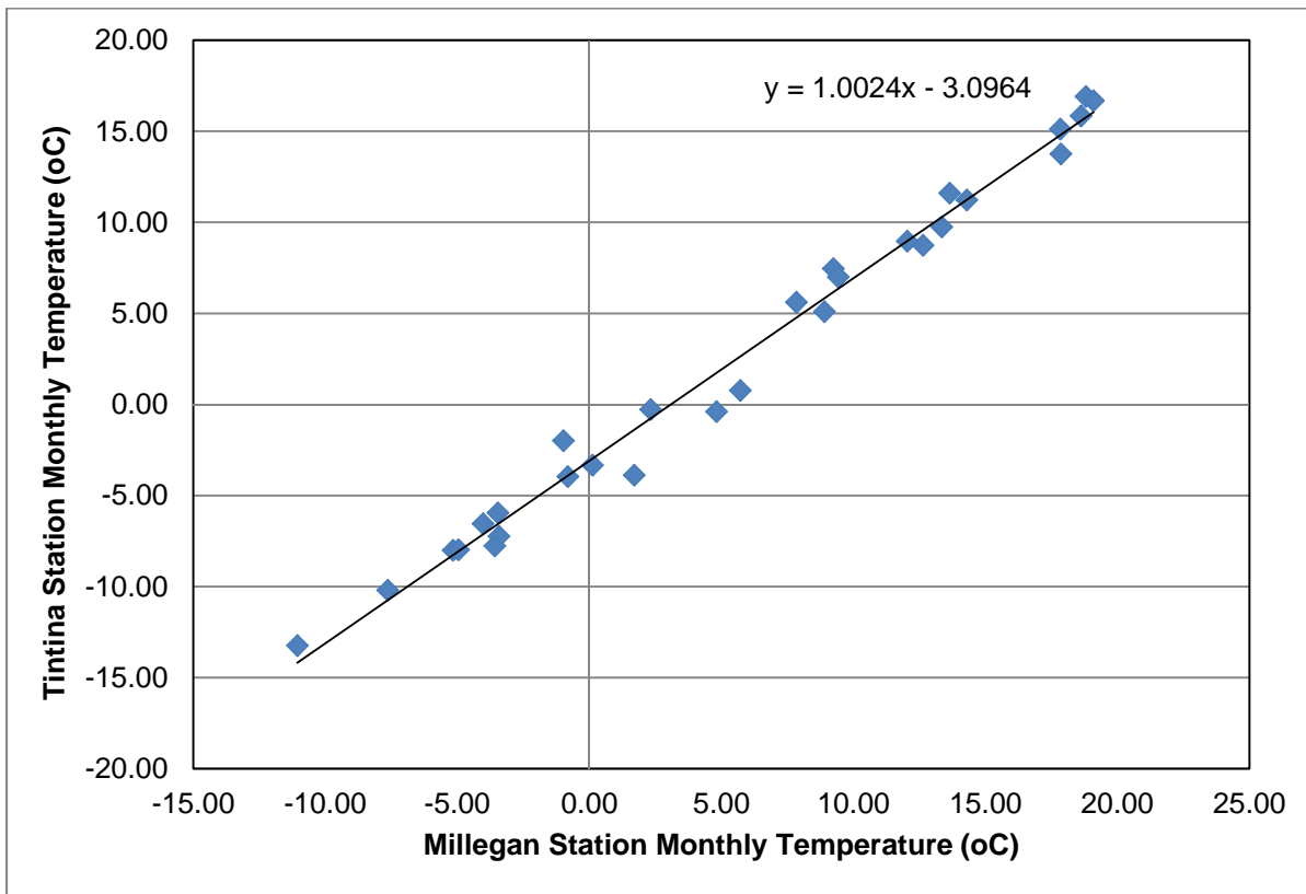
Figure 5 Tintina-Millegan Temperature Regression
